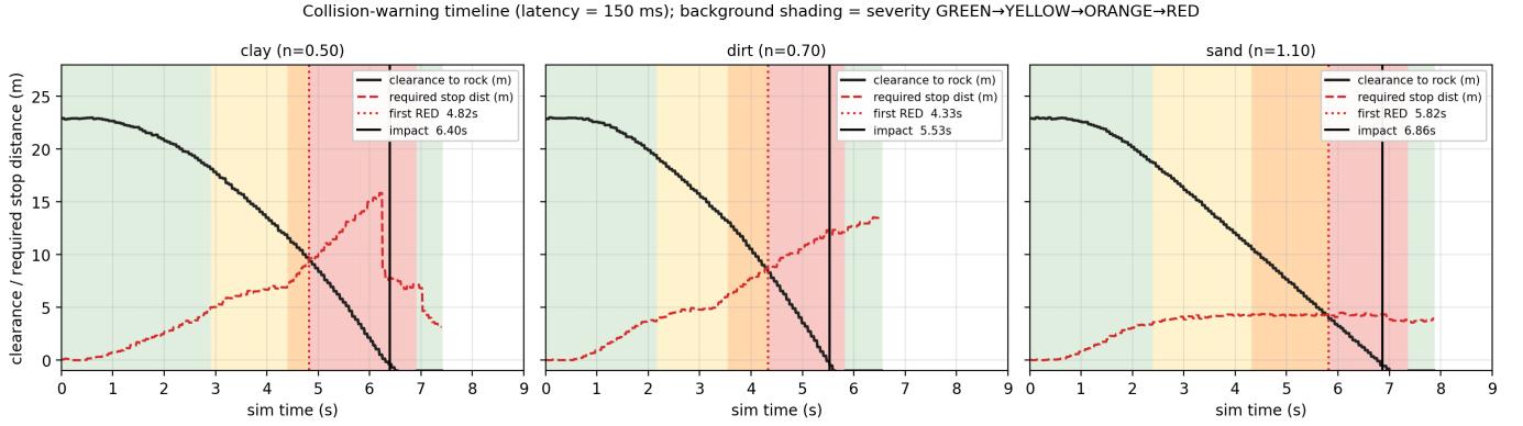
Fig. 25: Severity escalation over time for one representative blind-drive run per terrain at 150 ms one-way delay. Background shading is the live severity band (GREEN → YELLOW → ORANGE → RED); curves are the chassis clearance to the rock (solid) and the warning system’s running stopping-distance estimate (dashed). The first RED fires when the clearance curve drops to the stopping-distance curve.
