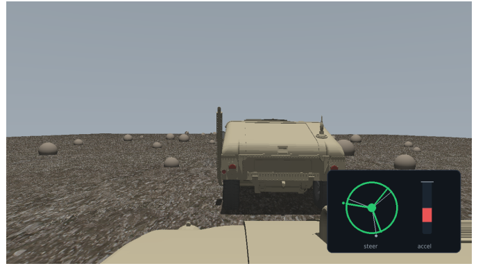
Fig. 16: The human-in-the-loop operator view: the Chrono::Sensor driver point-of-view over the SCM deformable terrain and boulder field (the same camera feed that carries the downlink latency), with the live HUD ( hil_hud.py ) overlaying the steering and throttle/brake state — the ghost mark is the delayed operator command, the solid mark the filtered command sent to the vehicle. The pipeline is a demonstrated capability; the quantitative safety result is obtained from the deterministic counterfactual of Sec. VII-F, not from human rounds.
