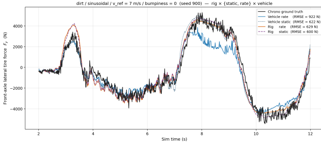
Fig. 5: One representative scenario from the four-way comparison (dirt, sinusoidal, v_{\text{ref}} = 7 m/s, b = 0 ), front-axle F_y . Black is Chrono ground truth; the four coloured traces are the deployed vehicle rate surrogate (light blue), the vehicle static surrogate (dark blue dotted), rig rate (orange), and rig static (purple dashed). Vehicle rate consistently under-predicts the peaks; the rig variants over-predict the same peaks; both static checkpoints track the envelope most tightly. The deployed default still attains the lowest RMS CTE but at the cost of the largest force-RMSE.
