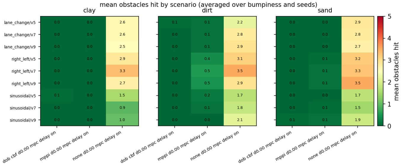
Fig. 23: 5G-profile latency compensation sweep: per-scenario collisions. Aggregate KPIs are in Table XIX.
