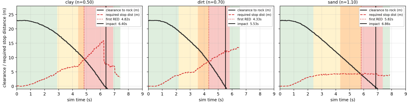
Fig. 25: Severity escalation over time for one representative blind-drive run per terrain at 150 ms one-way delay. Background shading is the live severity band (GREEN → YELLOW → ORANGE → RED); curves are the chassis clearance to the rock (solid) and the warning system’s running stopping-distance estimate (dashed). The first RED fires when the clearance curve drops to the stopping-distance curve.
