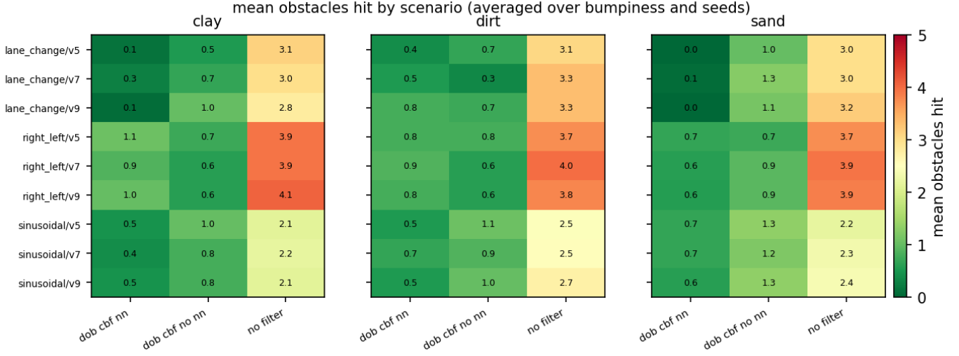
Fig. 18: DOB-CBF neural-surrogate ablation: per-scenario collisions. Aggregate KPIs are in Table XVI.
