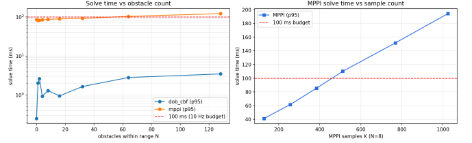
Fig. 23: Safety-filter solve time vs. obstacle count N (left) and MPPI sample count K (right), against the 100 ms / 10 Hz shield budget (dashed). DOB-CBF stays \leq 3.5 ms out to N = 128 ; MPPI is rollout-bound — flat in N , linear in K . Standalone solve timing, single-thread BLAS.
