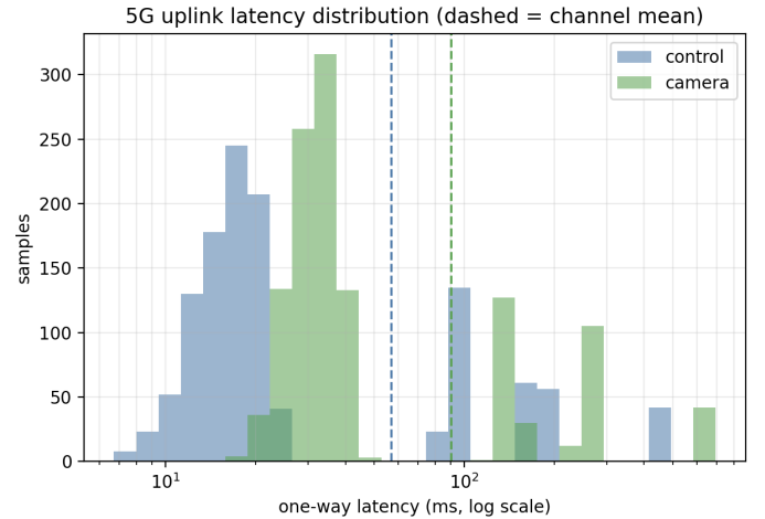
Fig. 23: Learned N-HiTS 5G uplink profile applied to the camera and control channels (log- x histogram; dashed lines are channel means). The profile is bimodal: a low-latency bulk (control around 10–25 ms, camera around 30–50 ms), a higher-latency cluster near 100–200 ms, and discrete outage spikes at 450 ms (control) and 660 ms (camera). Mean one-way latency is approximately 57 ms (control) and 91 ms (camera).
