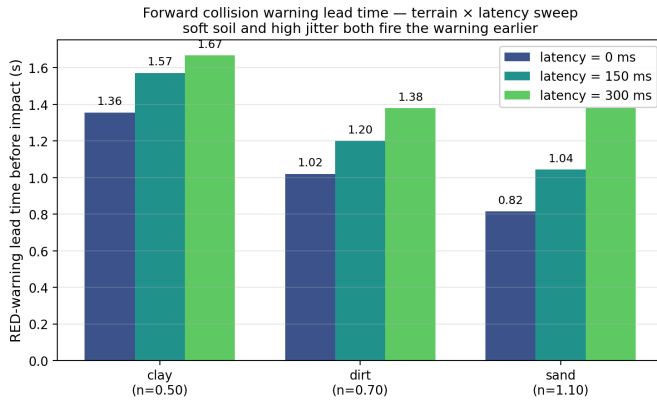
Fig. 27: Forward collision warning lead time before impact in the blind-drive sweep (no MPC, no safety filter, fixed throttle into a single rock). Both the terrain-conditioned brake budget and the latency-conditioned operator-reaction budget enlarge the required stopping distance and therefore advance the first RED warning: soft soil (clay) gets the longest lead, and within every terrain the lead grows monotonically with the configured one-way delay.
