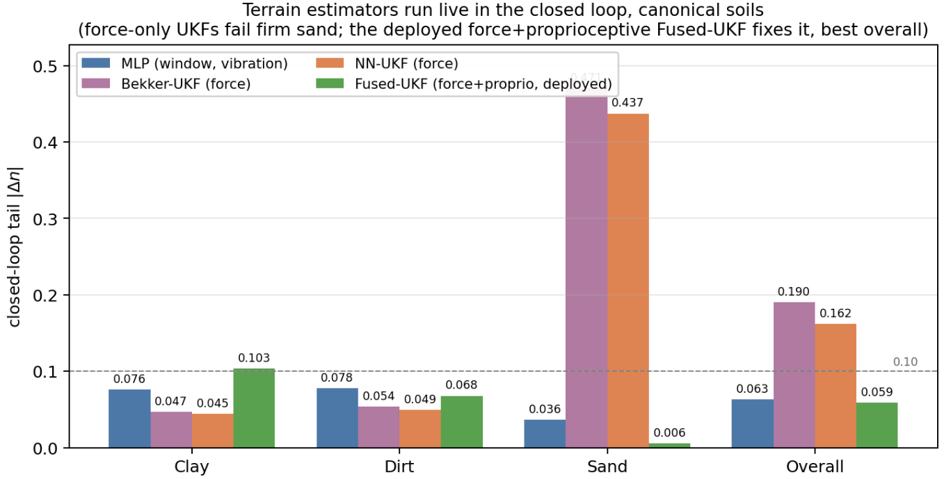
Fig. 10: Per-terrain closed-loop comparison of the four estimators on the canonical Chrono SCM presets — clay, sandy loam (dirt), dry sand — run live in the loop at v \in \{5, 7\} m/s, three seeds, 0.6 rad steering, tail |\Delta n| . The Bekker-UKF and force-only NN-UKF are most accurate on the soft soils but fail on firm sand ( |\Delta n| \approx 0.44 – 0.47 , an observability limit, cf. Fig. 9); the proprioceptive MLP is balanced; the deployed Fused-UKF recovers firm sand to 0.006 at the cost of being least accurate on soft clay (0.103).
