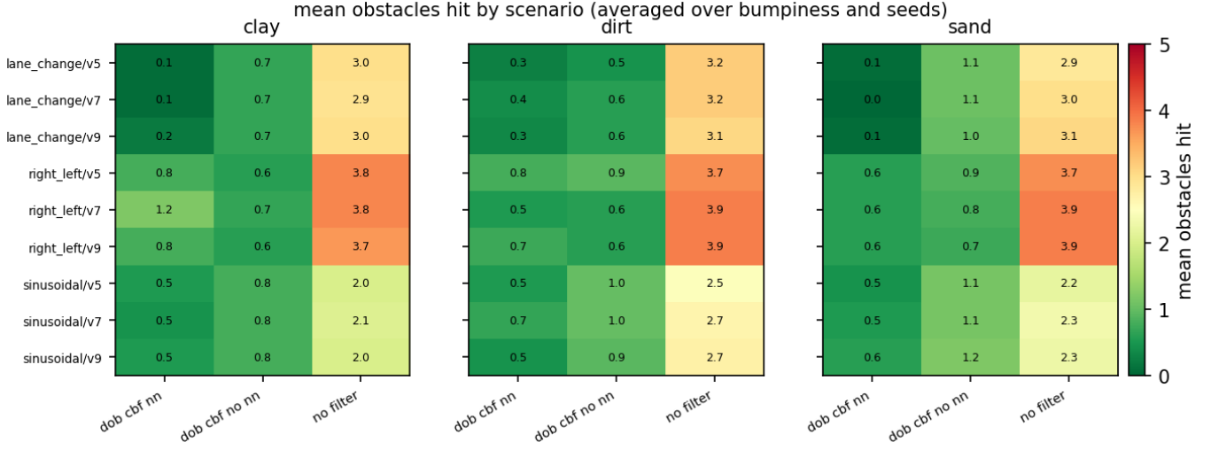
Fig. 19: DOB-CBF neural-surrogate ablation: per-scenario collisions. Aggregate KPIs are in Table XVI.
