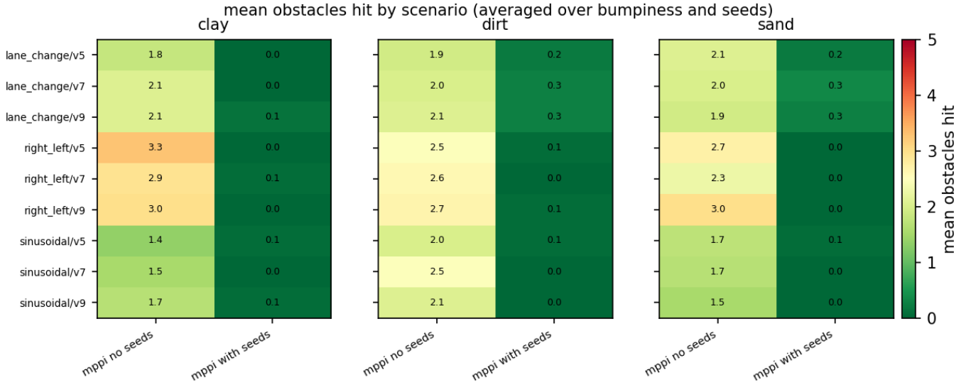
Fig. 20: MPPI seed-trajectory ablation. Removing the seeds eliminates the safety filter’s commitment to evasive maneuvers; the weighted mean then averages over many comparably high-error samples rather than concentrating on a recoverable trajectory.
