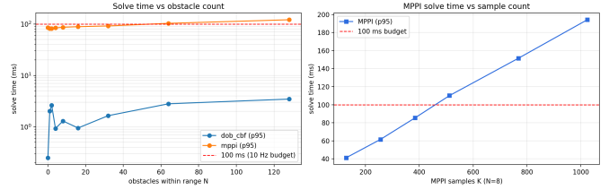
Fig. 23: Safety-filter solve time vs. obstacle count N (left) and MPPI sample count K (right), against the 100 ms / 10 Hz shield budget (dashed). DOB-CBF stays \leq 3.5 ms out to N = 128 ; MPPI is rollout-bound — flat in N , linear in K . Standalone solve timing, single-thread BLAS.
