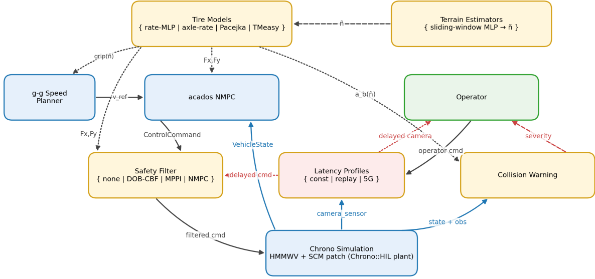
Fig. 1: Shared-control framework. Yellow nodes are in-process swap points resolved by the corresponding registry; blue/green nodes are process-boundary or operator endpoints. Solid arrows are runtime data flow over ZeroMQ; dashed arrows are the latency-affected operator paths; dotted arrows are tire-surrogate queries (build-time CasADi export plus per-tick safety-filter rollouts).
