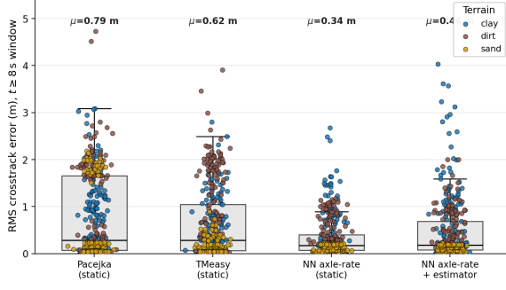
Fig. 3: Same benchmark, RMS CTE distribution per variant. Box plots show interquartile range and median across all 405 runs per variant; jittered scatter points are coloured by terrain (clay, dirt, sand). The two analytical baselines (Pacejka, TMeasy) carry long right tails driven by a few dirt cases at higher v_{\text{ref}} ; both neural variants compress the distribution sharply. The estimator-on variant nearly matches the matched-prior static row, the deployable claim of Sec. III-C.
