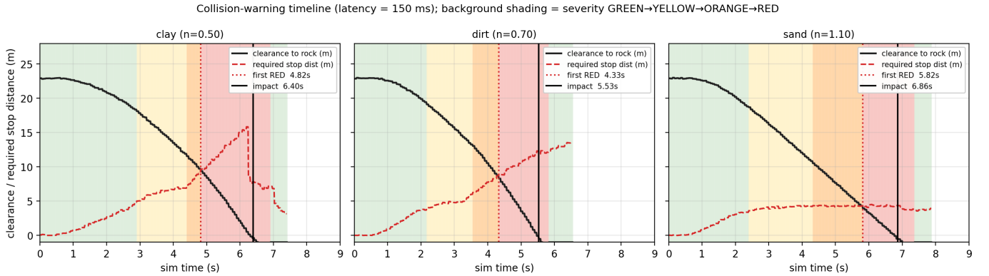
Fig. 27: Severity escalation over time for one representative blind-drive run per terrain at 150 ms one-way delay. Background shading is the live severity band (GREEN \rightarrow YELLOW \rightarrow ORANGE \rightarrow RED); curves are the chassis clearance to the rock (solid) and the warning system’s running stopping-distance estimate (dashed). The first RED fires when the clearance curve drops to the stopping-distance curve.
