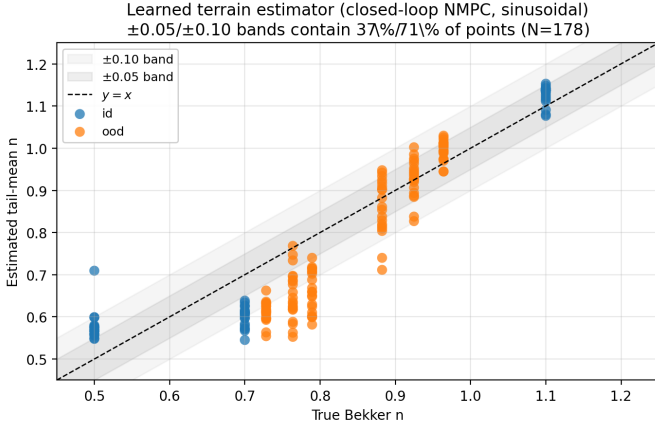
Fig. 6: Learned (sliding-window MLP) terrain estimator: true vs. estimated Bekker n (tail-window mean) on the closed-loop sinusoidal benchmark, evaluated within the estimator's training envelope (bumpiness \in \{0, 4\} ). Blue = in-distribution canonical soils (clay/dirt/sand); orange = Bekker-jittered out-of-distribution soils ( n sampled in [0.40, 1.30] , other five Bekker parameters perturbed \pm 30\text{--}50\% ). The \pm 0.05 / \pm 0.10 bands around y = x contain 40% / 68% of points. The estimator tracks the diagonal across the deployment range, with a mild systematic over-prediction in the lowest- n (clay) bin (mean estimate 0.59 vs. true 0.50). See the out-of-envelope note in the text for behaviour at bumpiness 8.
