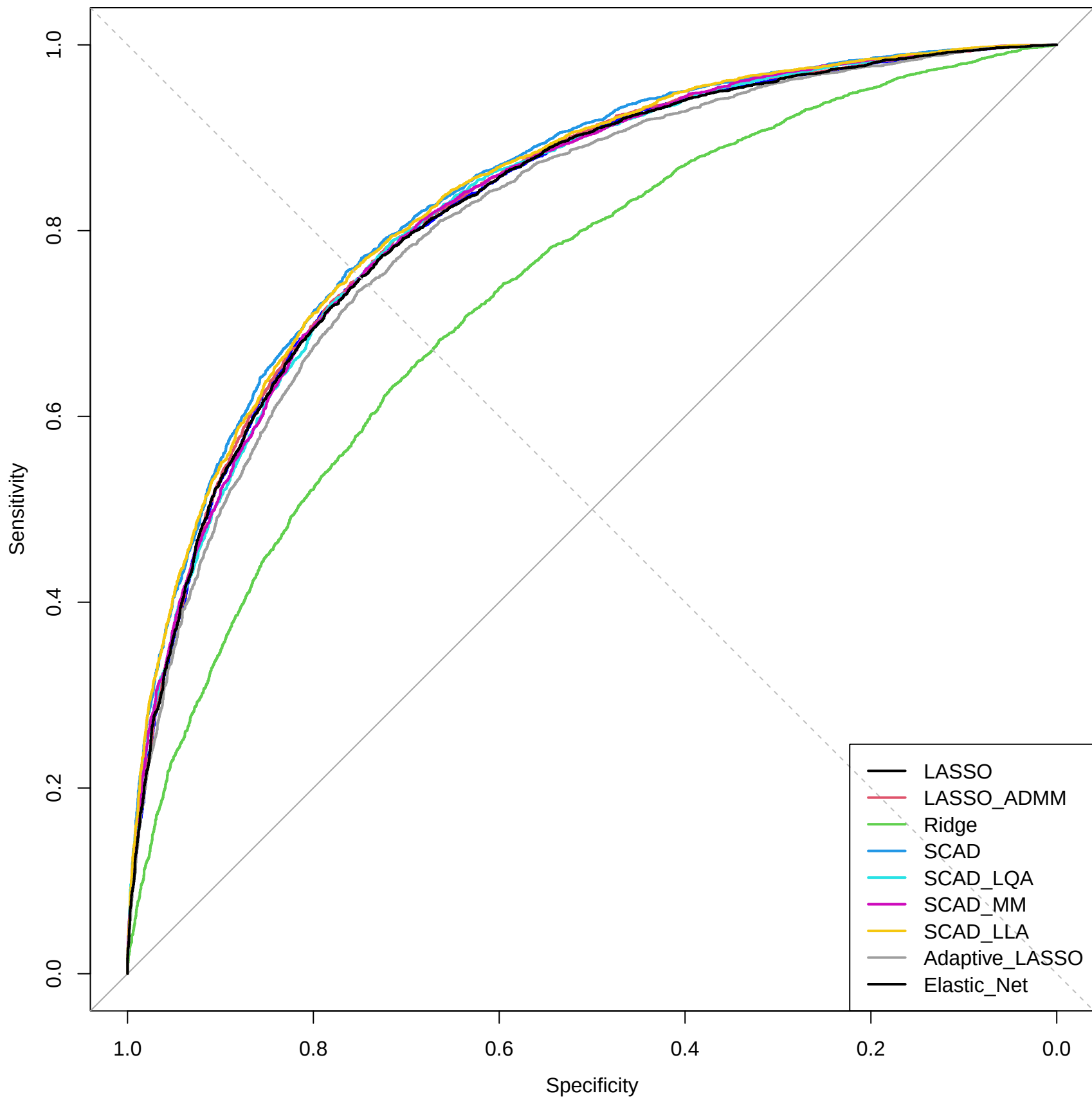
ROC Curves for Different Models( \rho=0.3 p=100 )
