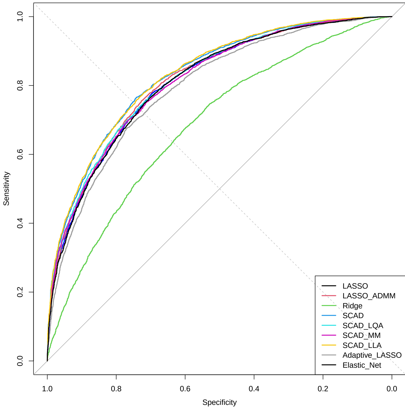
ROC Curves for Different Models( \rho=0.3 p=150 )
