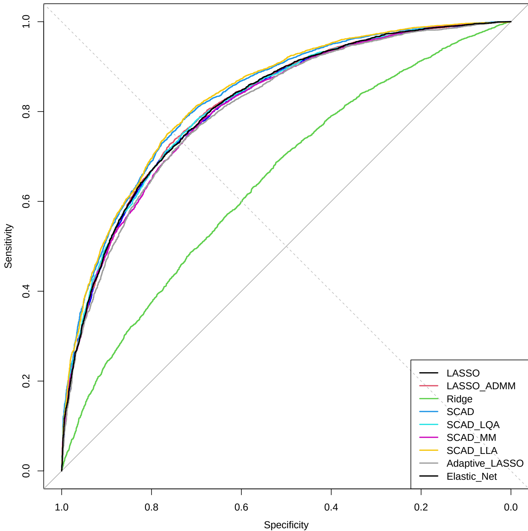
ROC Curves for Different Models( \rho=0.3 p=200 )
