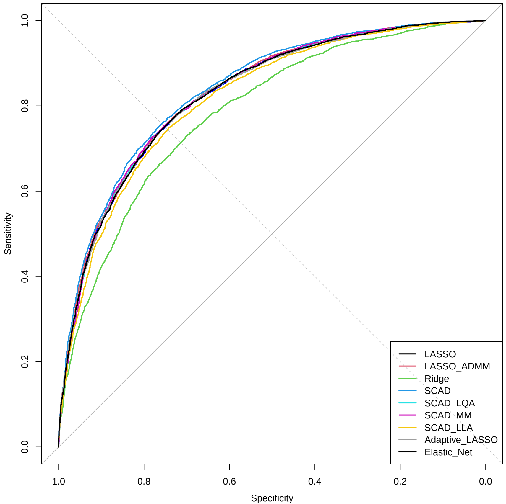
ROC Curves for Different Models( \rho=0.3 p=50 )
