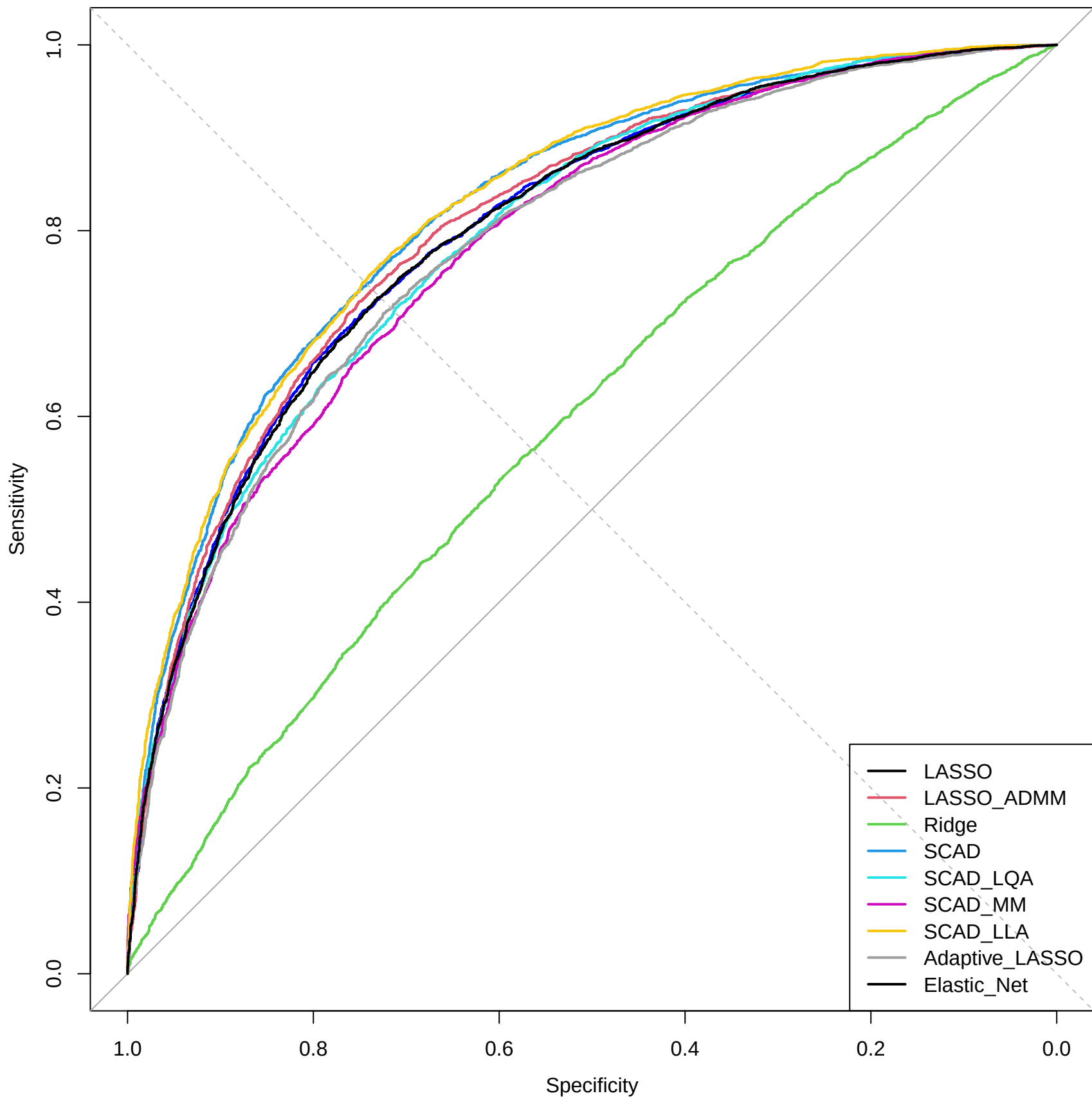
ROC Curves for Different Models( \rho=0.3 p=600 )
