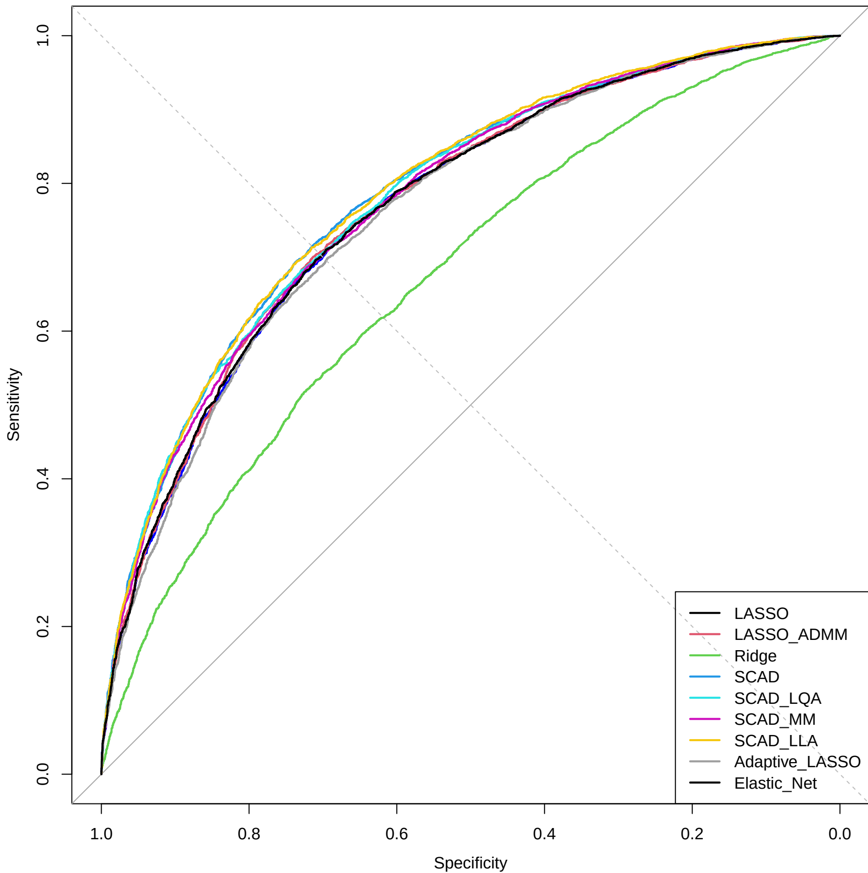
ROC Curves for Different Models( \rho=0.6 p=100 )
