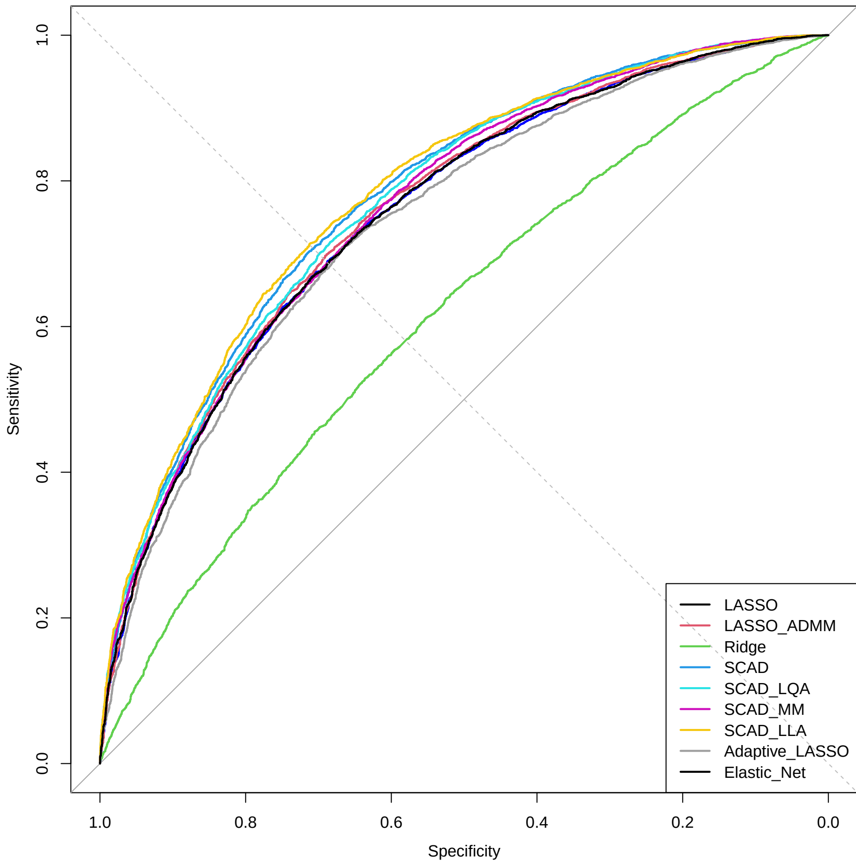
ROC Curves for Different Models( \rho=0.6 p=150 )
