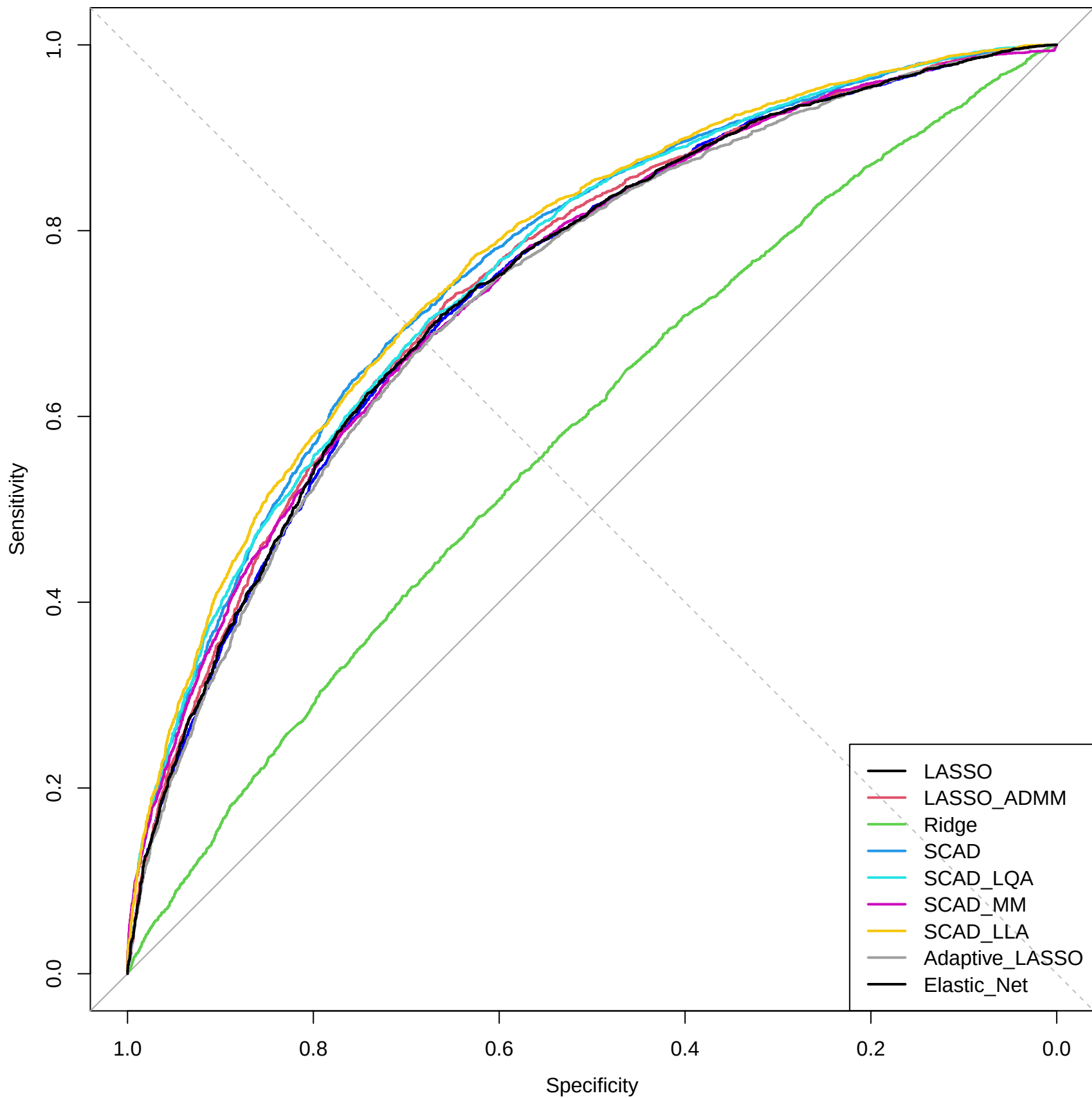
ROC Curves for Different Models( \rho=0.6 p=200 )
