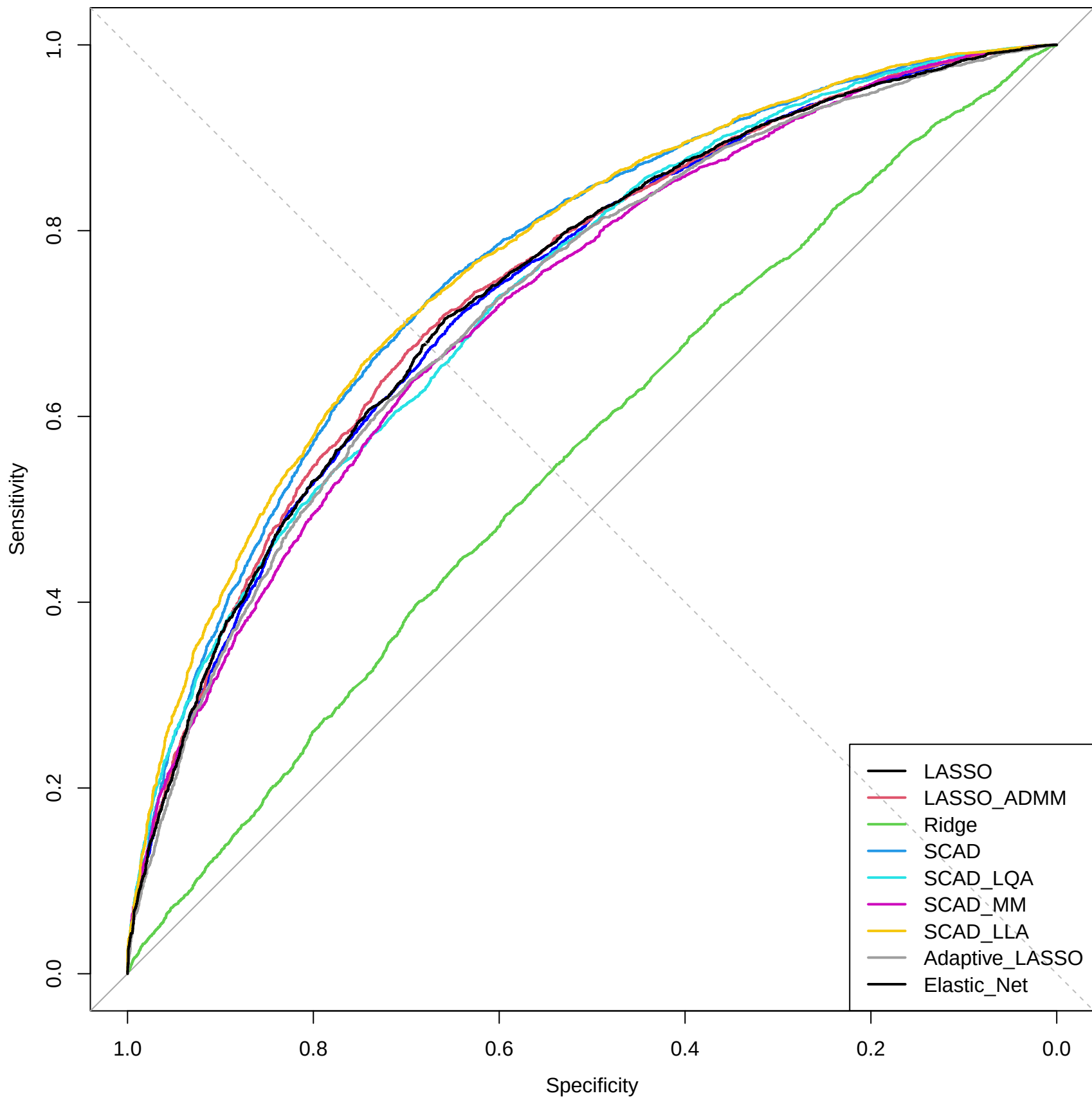
ROC Curves for Different Models( \rho=0.6 p=400 )
