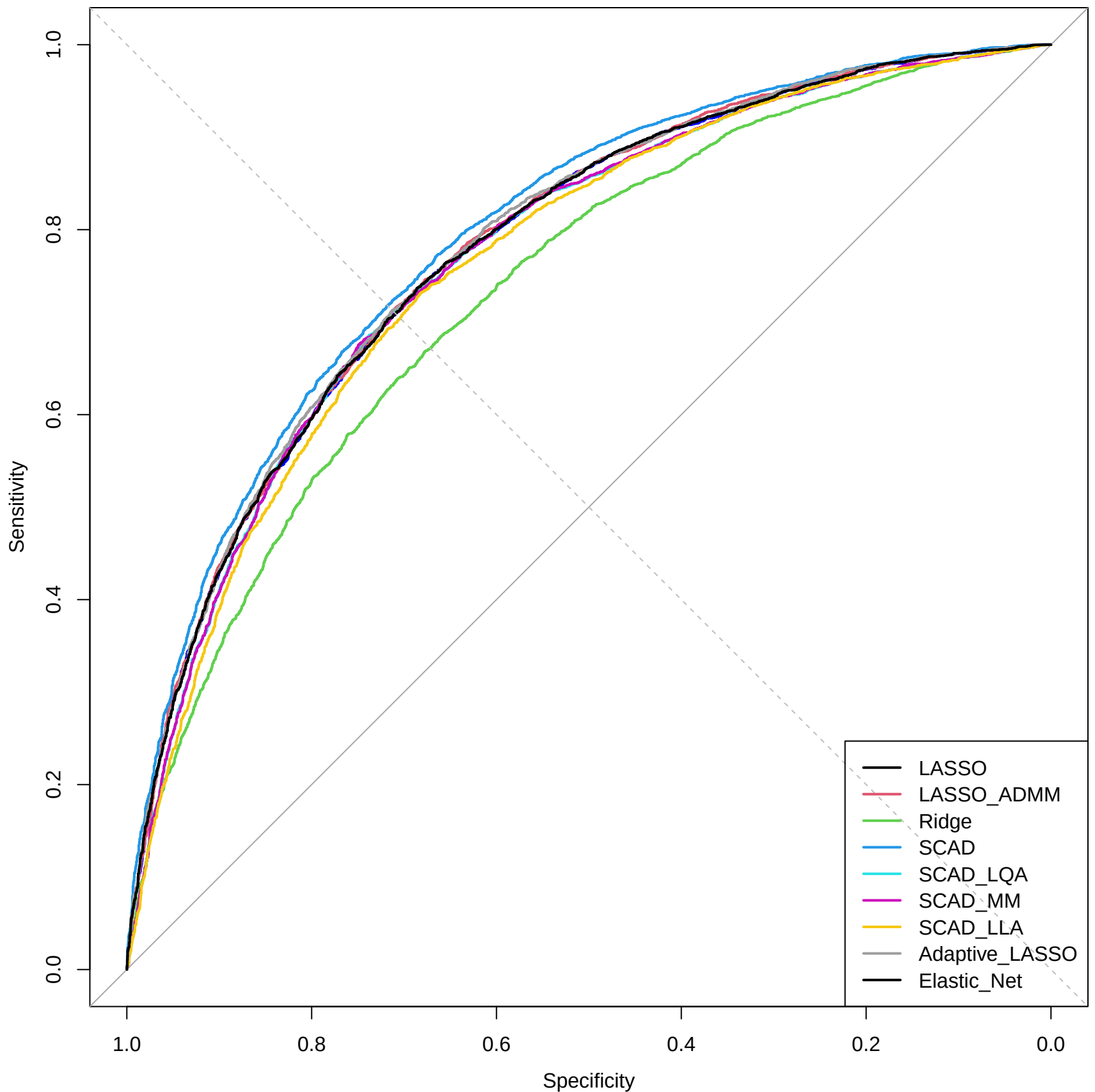
ROC Curves for Different Models( \rho=0.6 p=50 )
