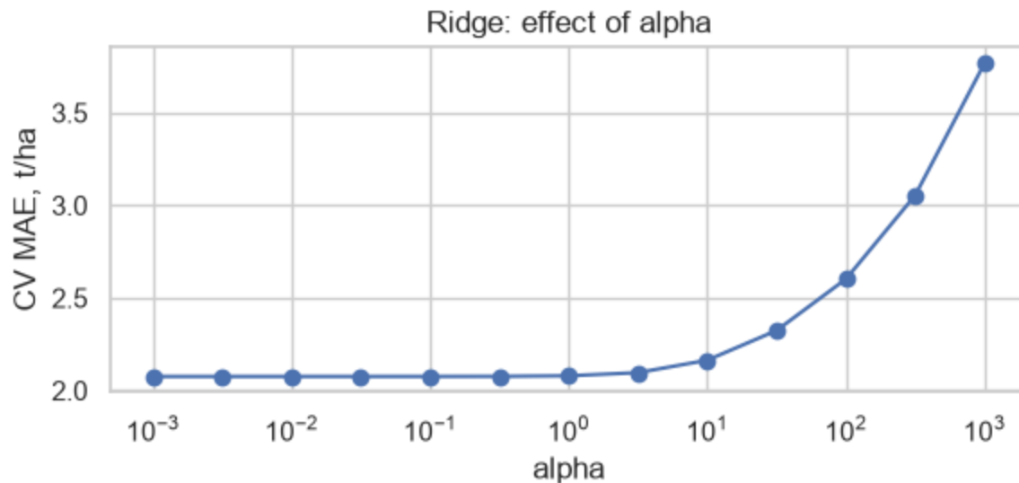
Figure 5. For \alpha \leq 1 the error does not change – the penalty is too small to matter. From \alpha \approx 10 the error grows fast because the coefficients are shrunk too much (underfitting). The best \alpha is the smallest one, so regularization does not help accuracy here.
