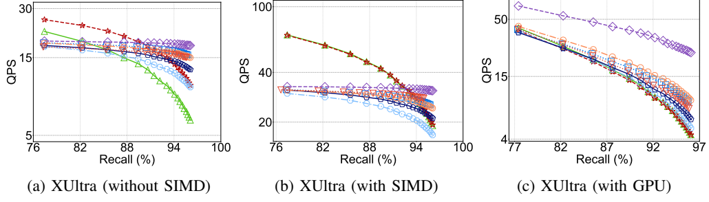
Fig. 19: Comparisons of DCO methods using the IVF index on XULtra dataset across different hardware environments
