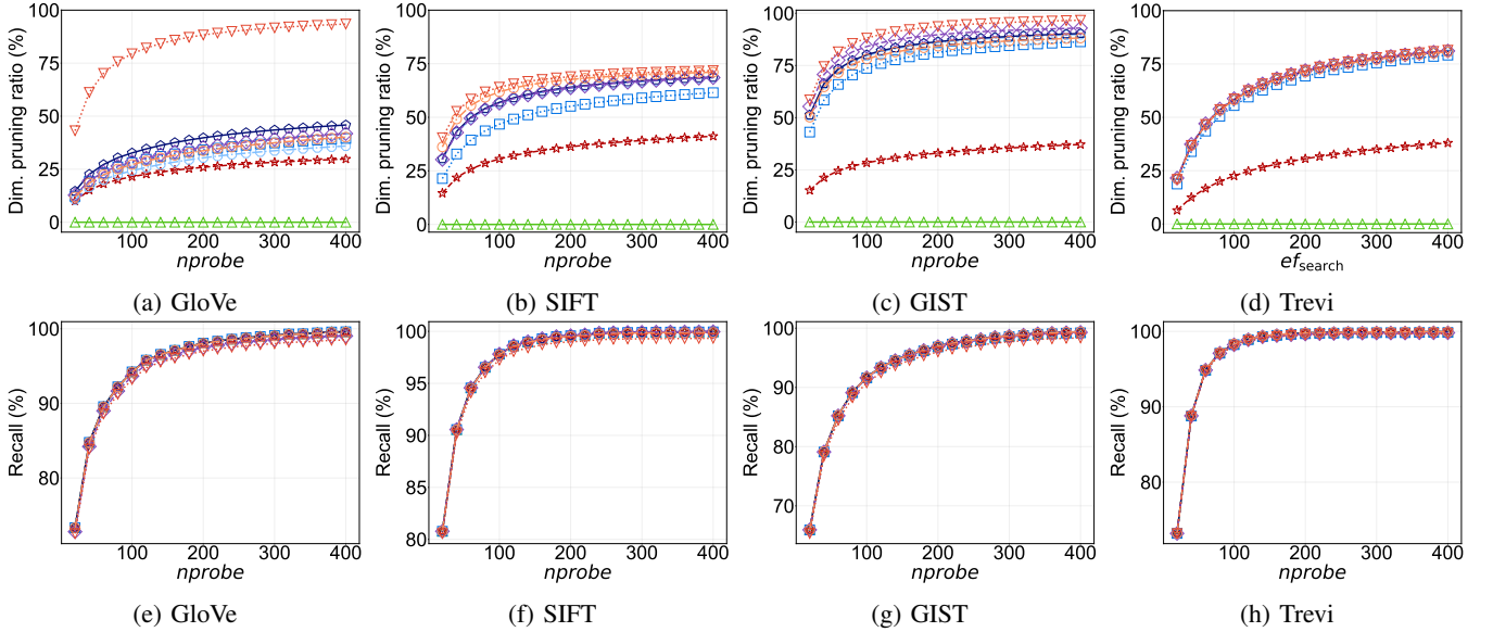
Fig. 20: Dimension pruning via DCO and its impact on recall on IVF
