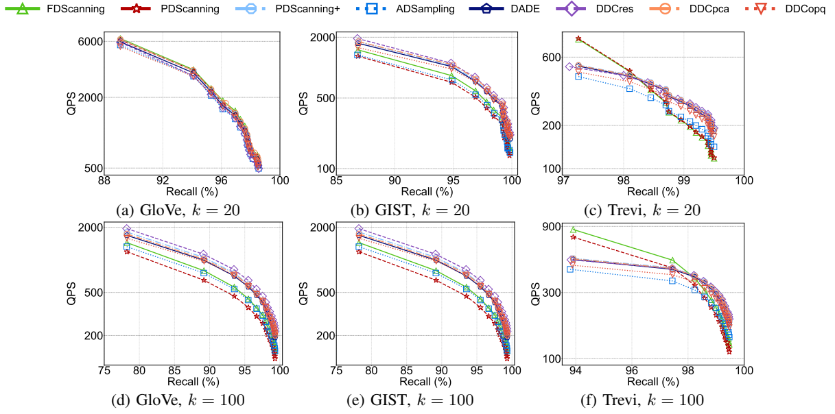
Fig. 18: Performance comparison on AVX2
