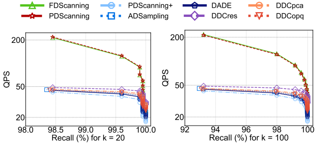
Fig. 5: Performance on ultra-high-dimensional dataset XULtra
