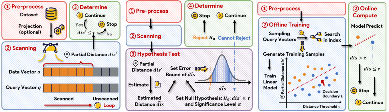
(a) Simple scanning based method
