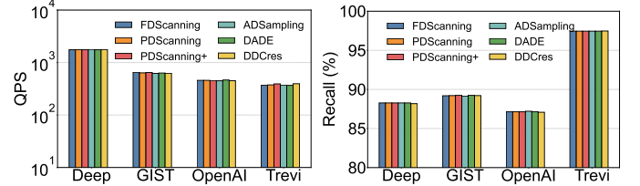
Fig. 10: Performance evaluation of different indexes
