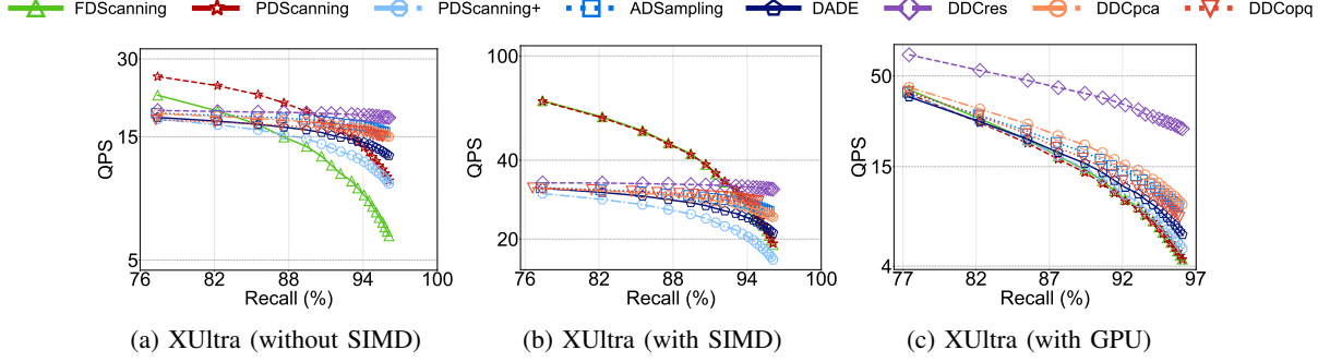
Fig. 17: Comparisons of DCO methods on the IVF index across different hardware environments
