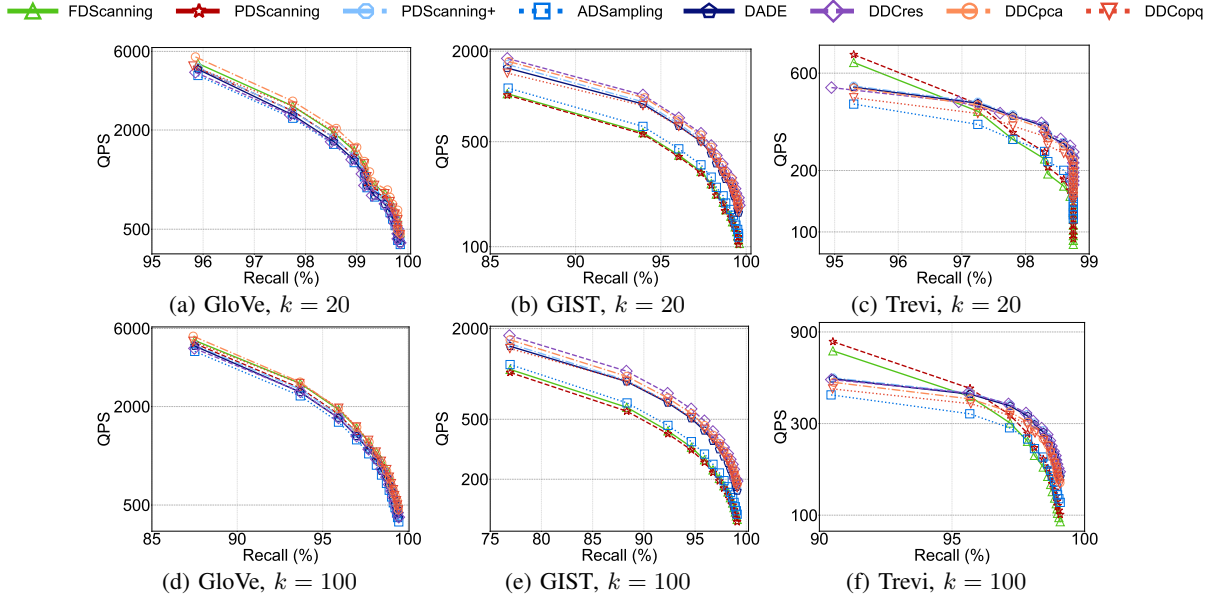
Fig. 19: Search performance using cosine similarity
