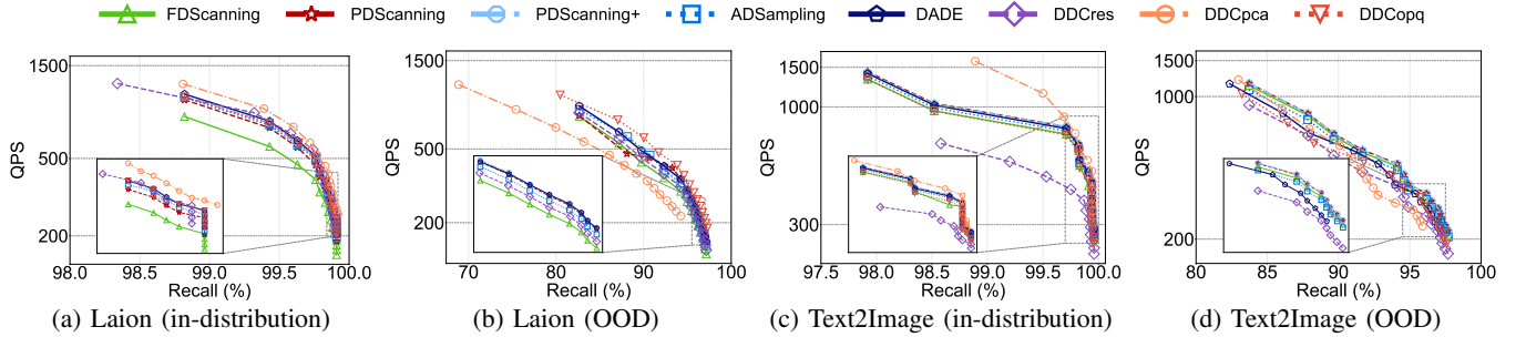
Fig. 18: Results on in-distribution and OOD queries without SIMD
