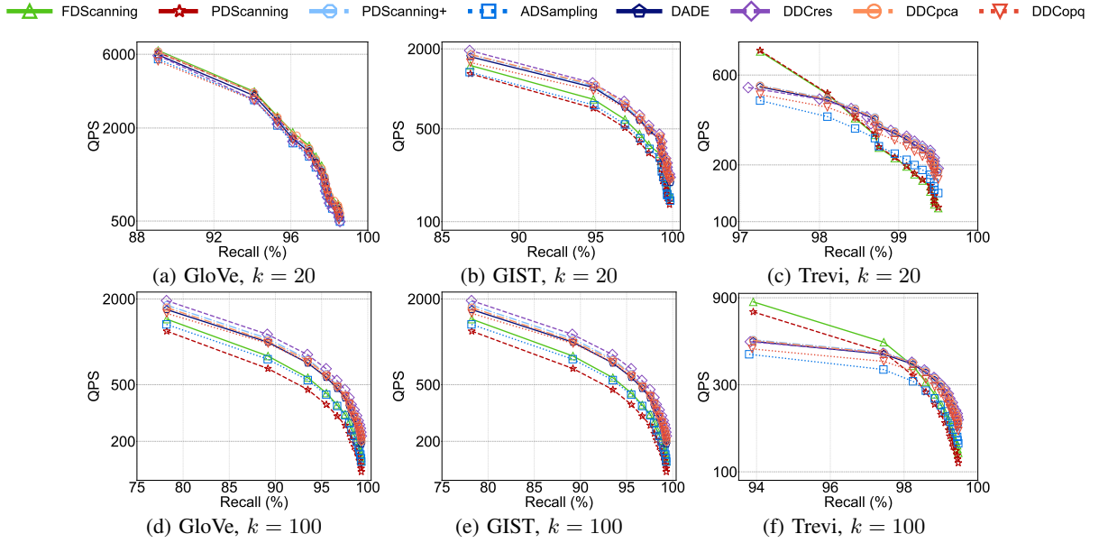
Fig. 20: Performance comparison on AVX2
