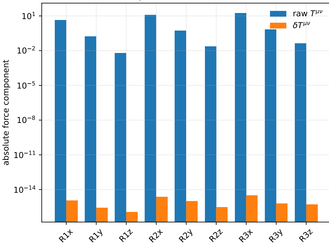
Analytic-wind force zero test
