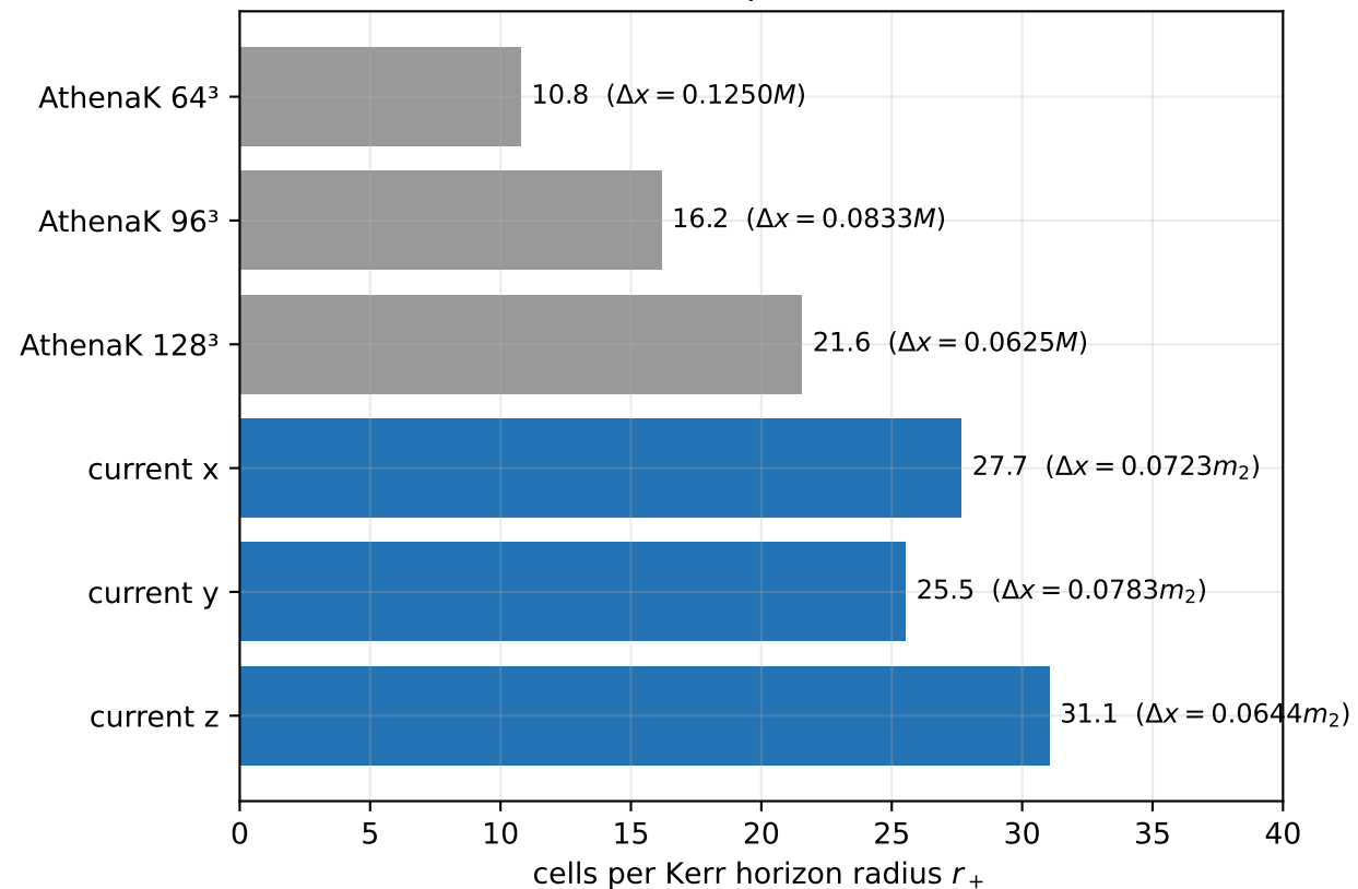
Near-horizon spatial resolution
