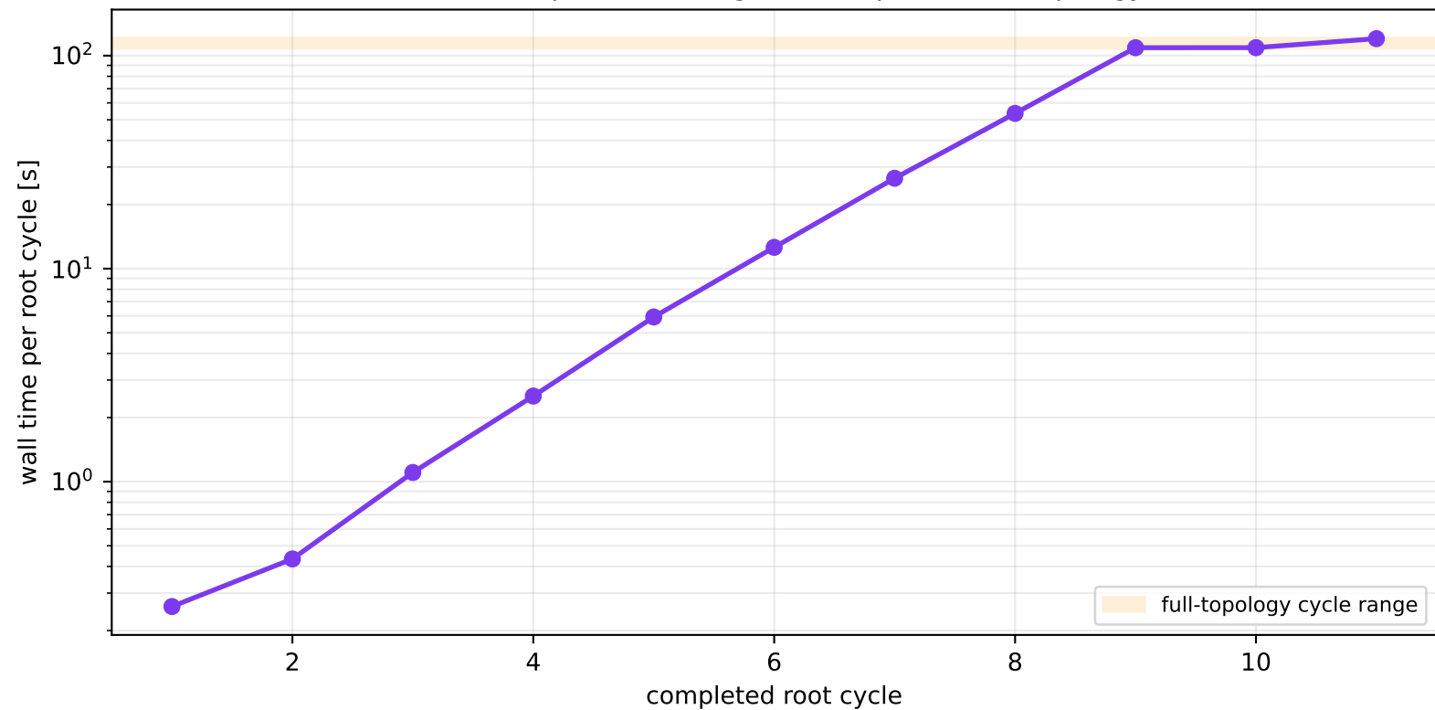
AMR startup cost converges to the production topology
