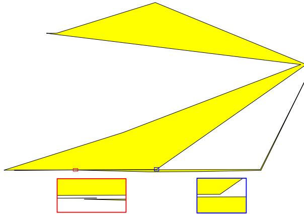
Figure 4: The intersection of \hat{S} with the plane y = 0 , which is the boundary of two simply-connected components colored in yellow. The boxes contain the manifold view of their respective regions in the original slice.
