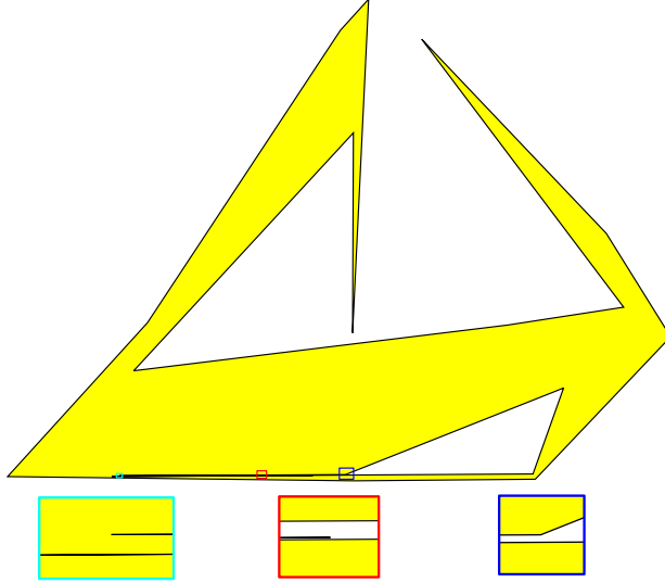
Figure 5: The intersection of \hat{S} with the plane x = 0 , which is the boundary of a region that is not simply-connected. Again, the boxes contain the manifold view of their respective regions in the original slice.
