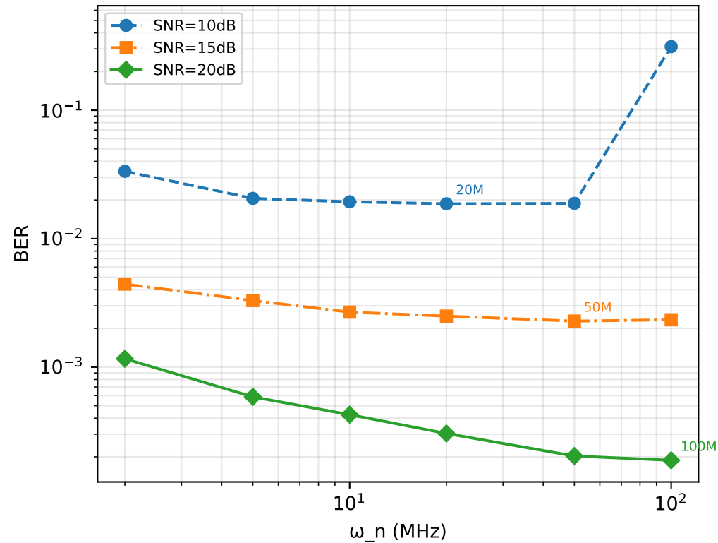
Weak Turbulence
