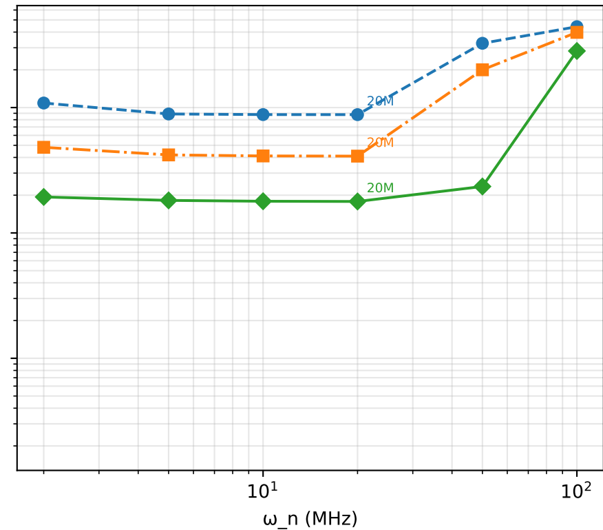
Strong Turbulence
