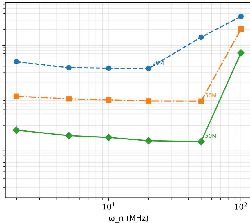
Moderate Turbulence
