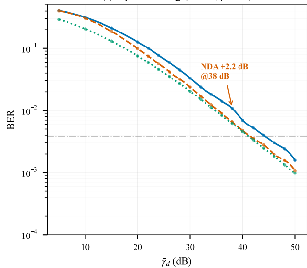
(f) Uplink strong ( \alpha=1.0, \beta=0.7 )
