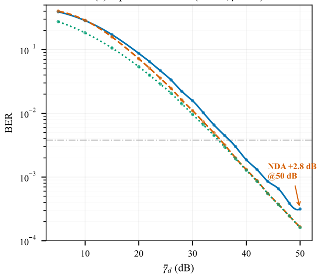
(e) Uplink moderate ( \alpha=1.2, \beta=0.9 )
