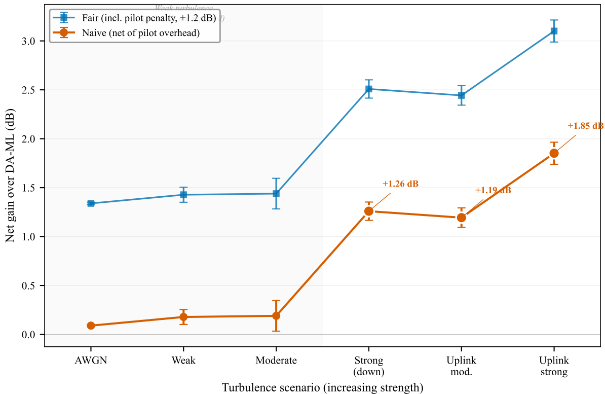
NDA-ML Net Gain vs. Turbulence Strength
