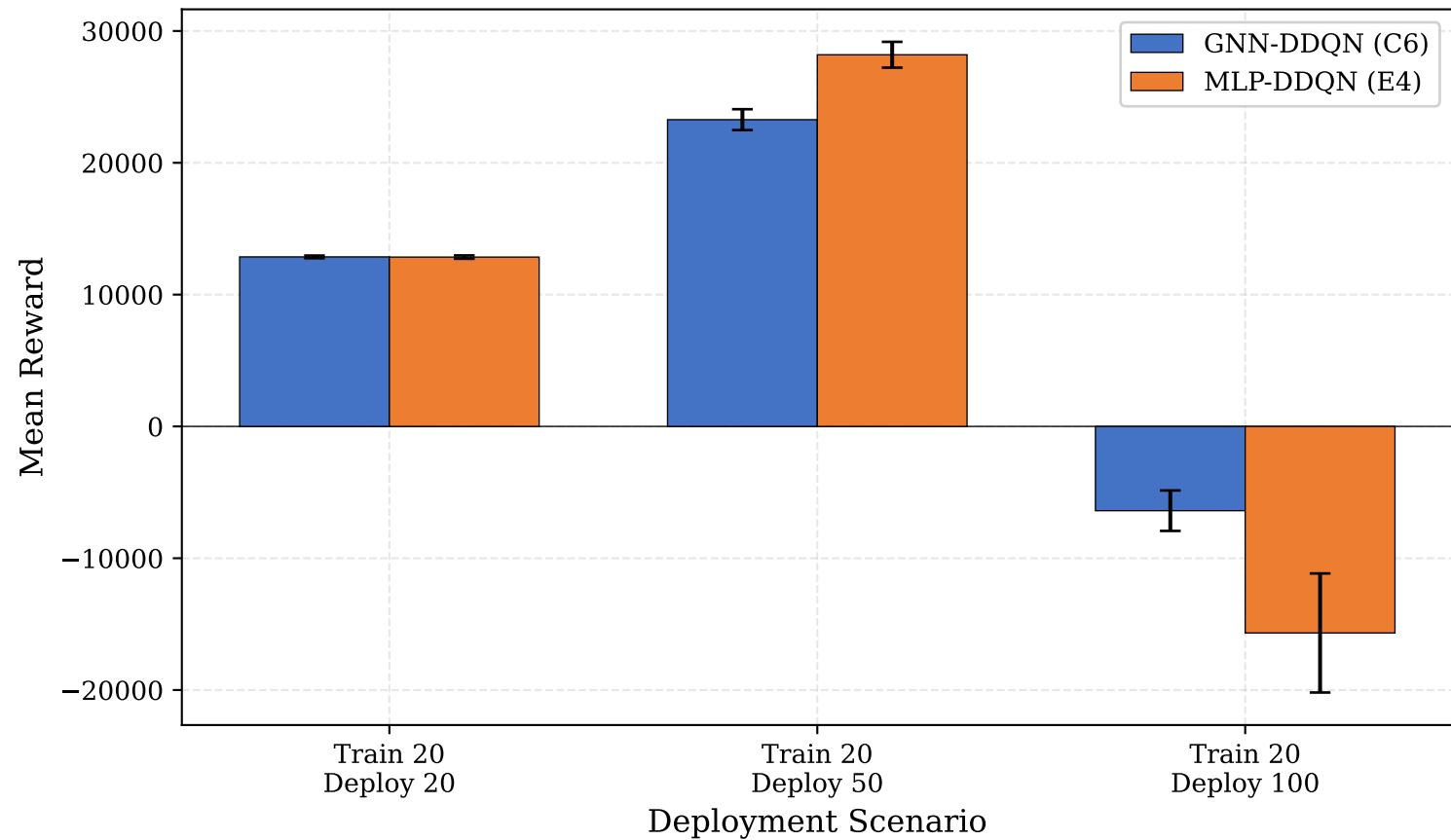
Ch2: Size Generalization Performance
