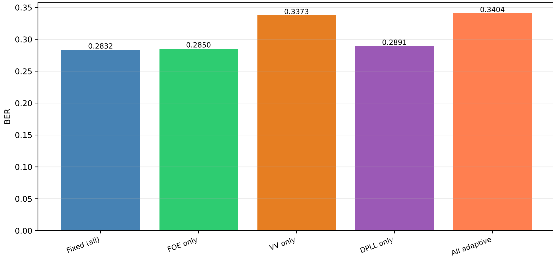
Ablation Study: Strong Turbulence, SNR=20dB
