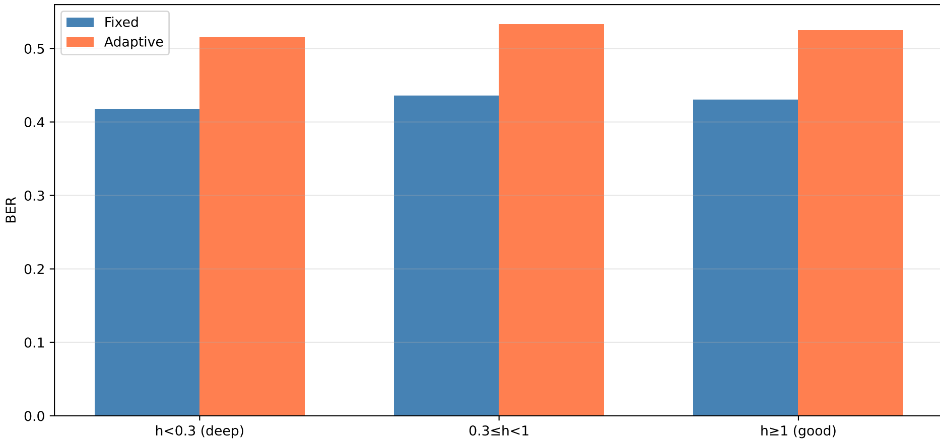
Block-level BER by Channel Gain (Strong Turbulence)
