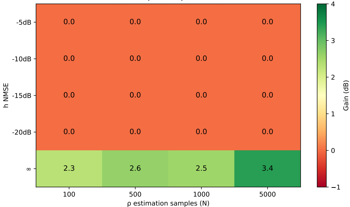
Pre-compensation Gain (dB) Weak turb, \tau=5\text{ms} , SNR=15dB
