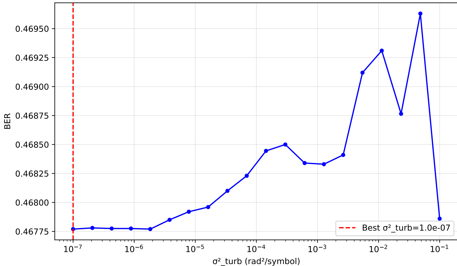
Q Matrix Grid Search (Strong turbulence, SNR=20dB)
