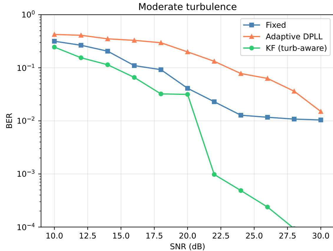
BER vs SNR: KF vs Baselines (f dot =150 MHz/s)
