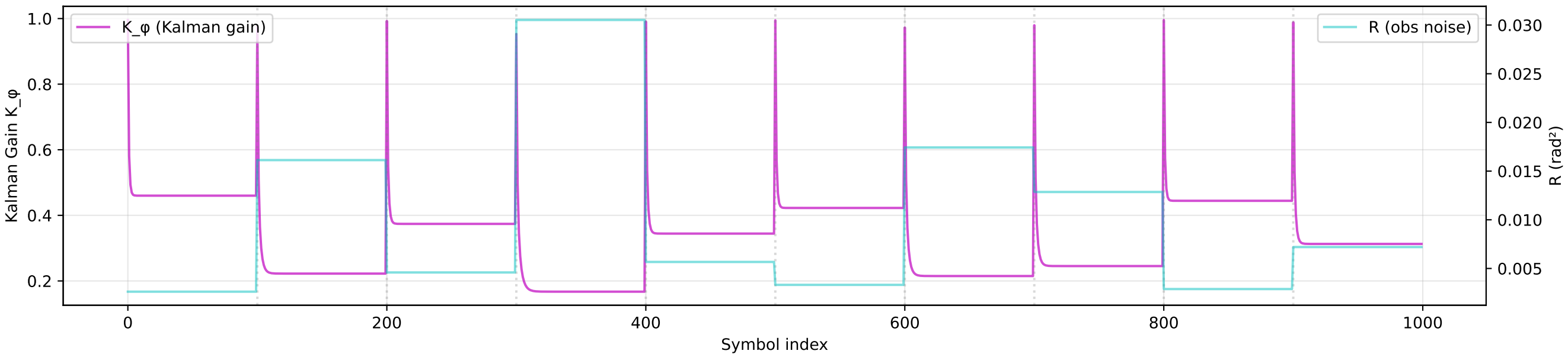
Kalman Gain & Observation Noise ( R \propto 1/h )
