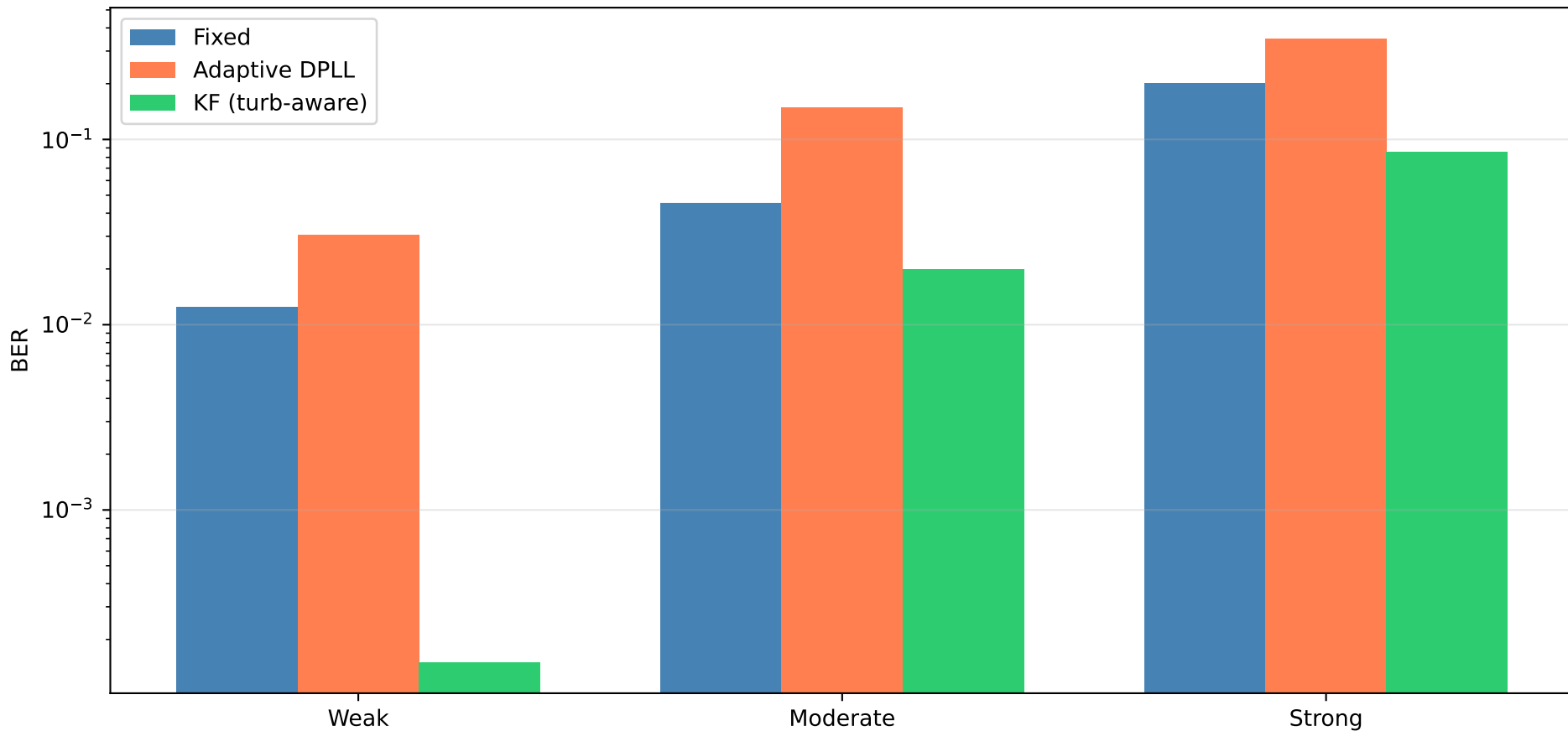
Carrier Sync Comparison: KF vs Baselines
