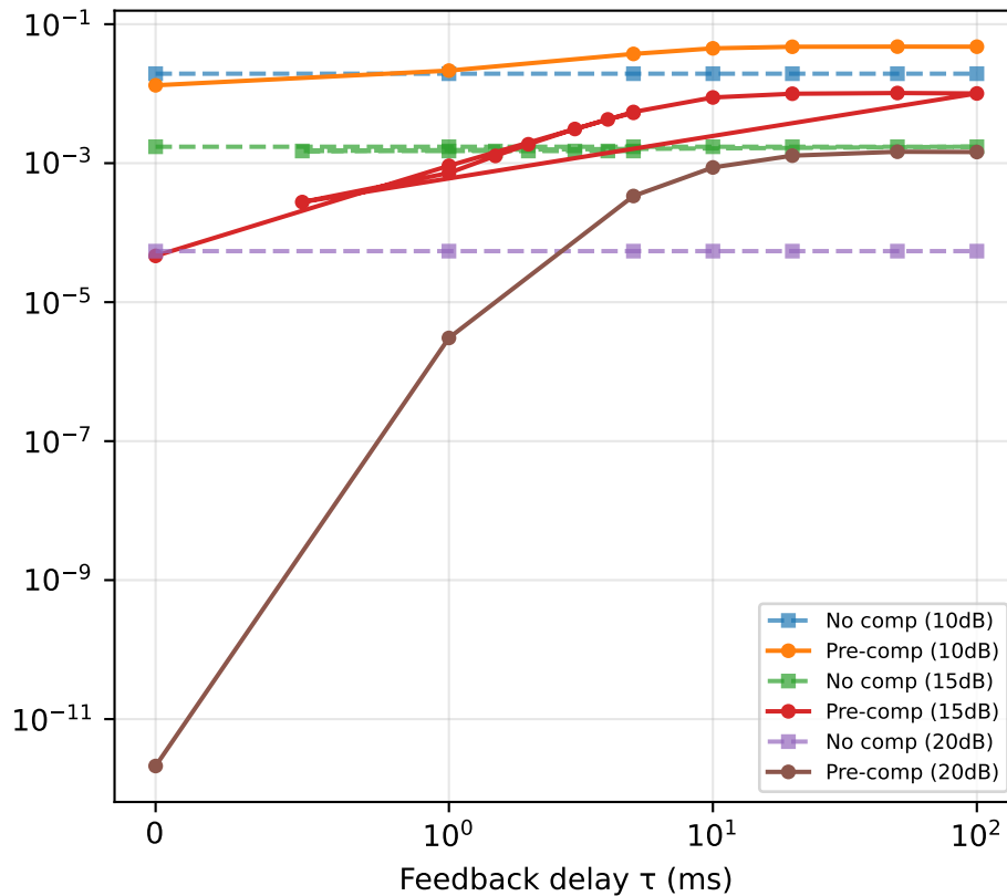
Moderate turbulence
