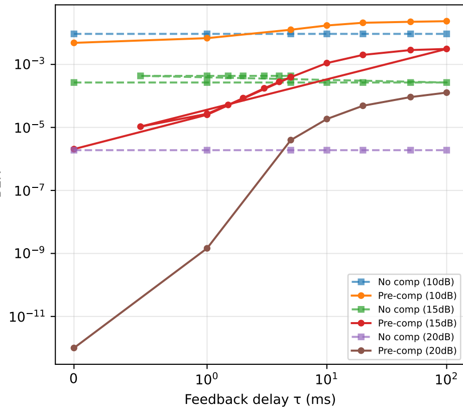
Weak turbulence
