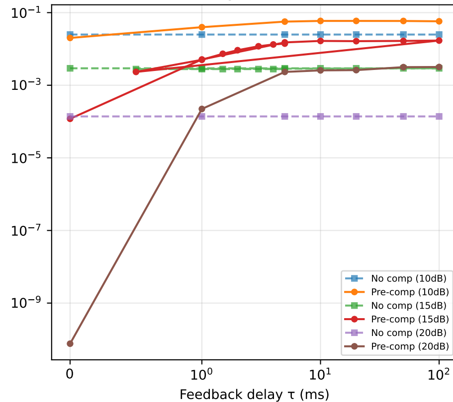
Strong turbulence
