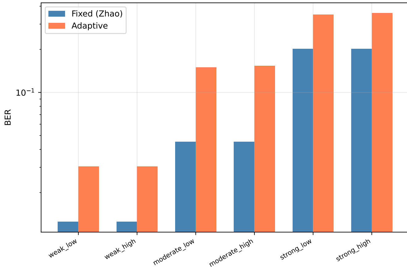
BER Comparison
