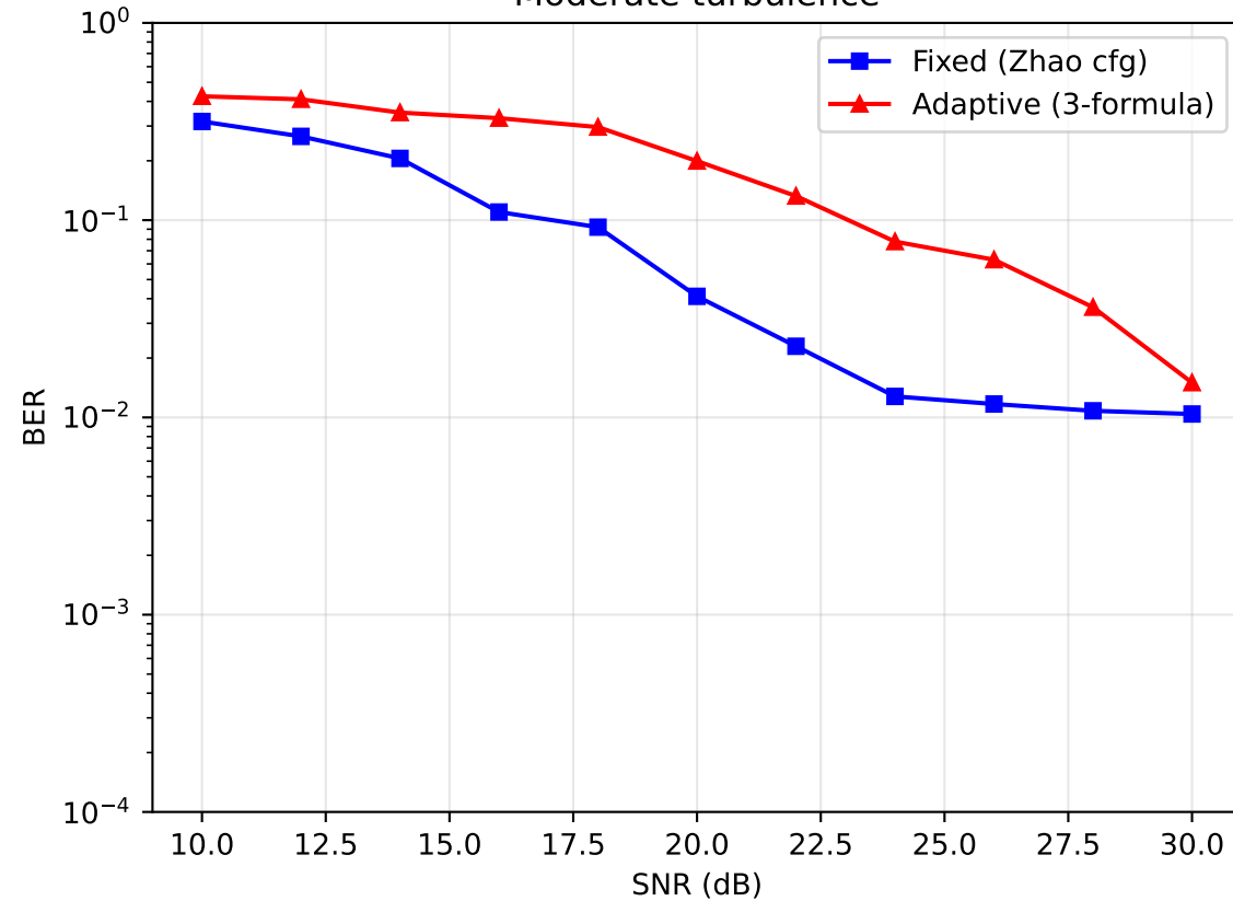
Moderate turbulence
