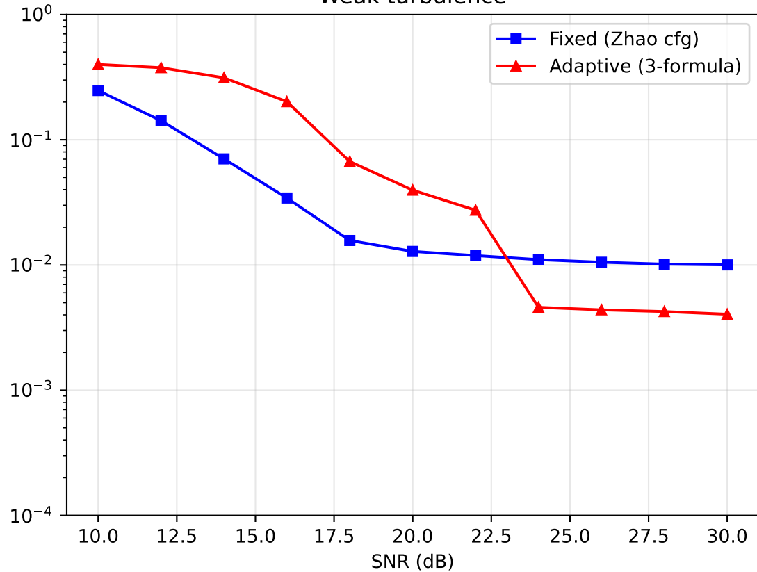
Weak turbulence
