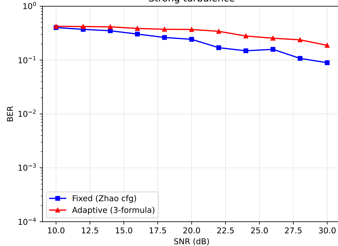
Strong turbulence
