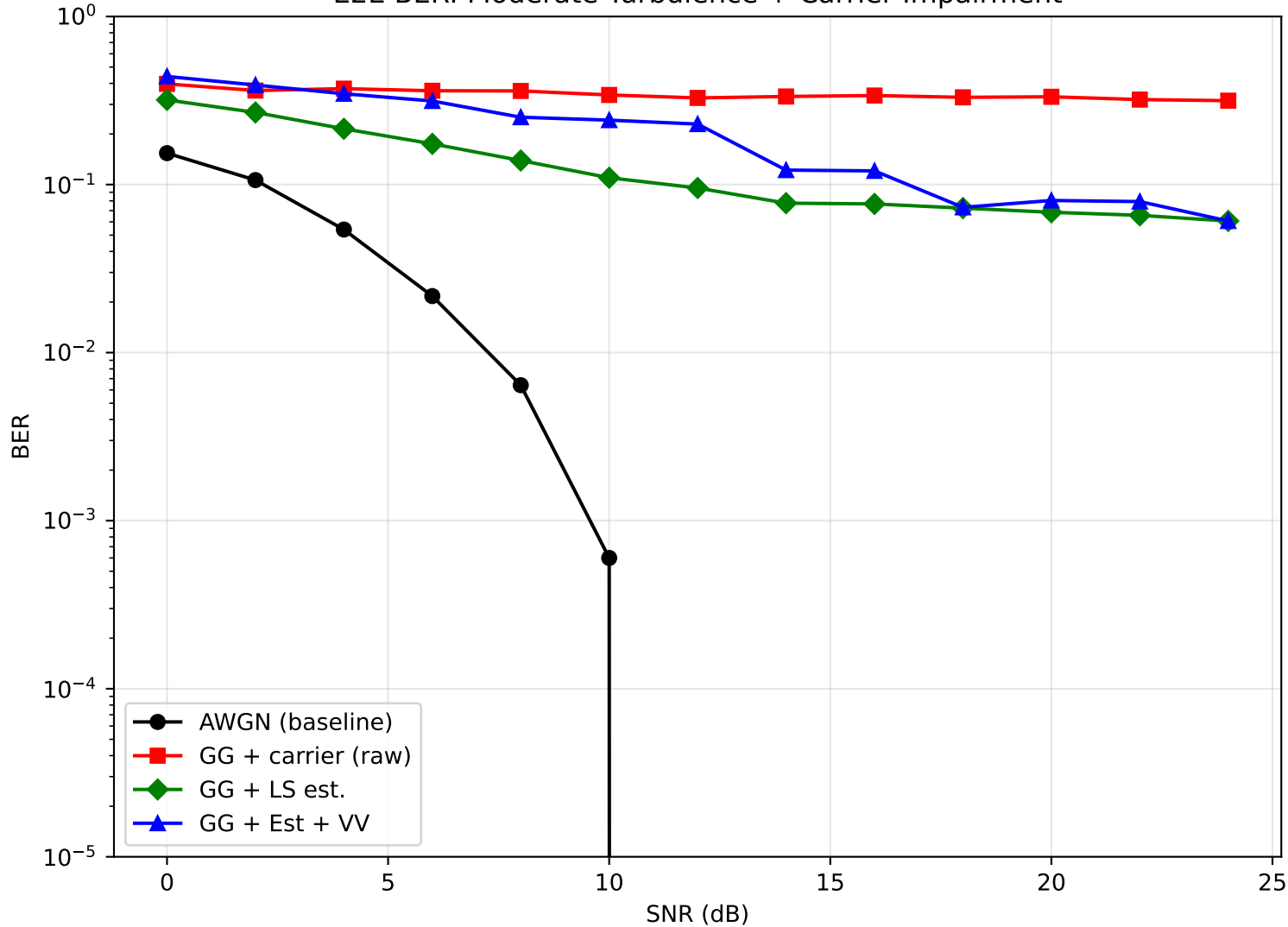
E2E BER: Moderate Turbulence + Carrier Impairment
