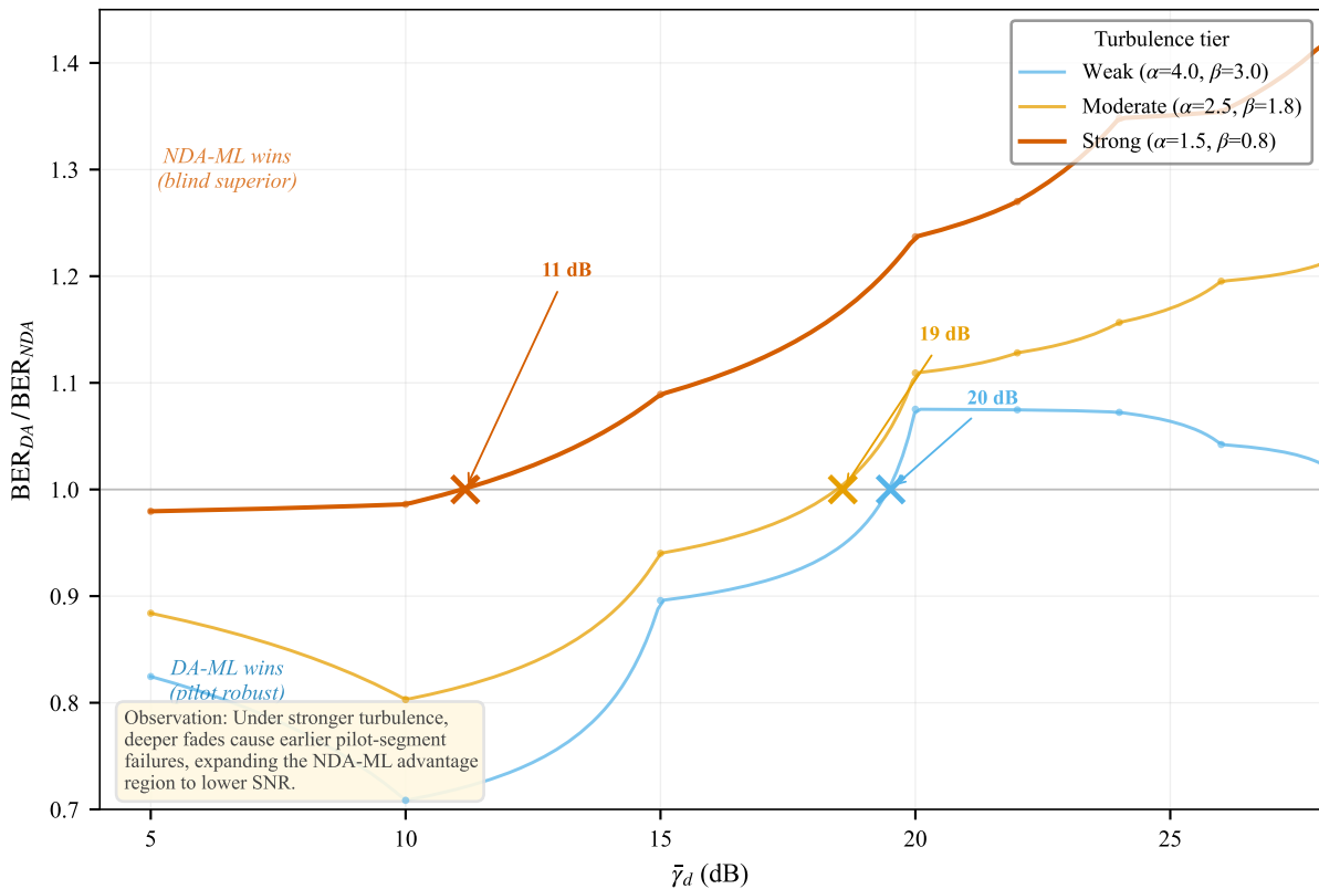
Crossover Shifts toward Lower SNR as Turbulence Strengthens (NDA Advantage Region Widens)
