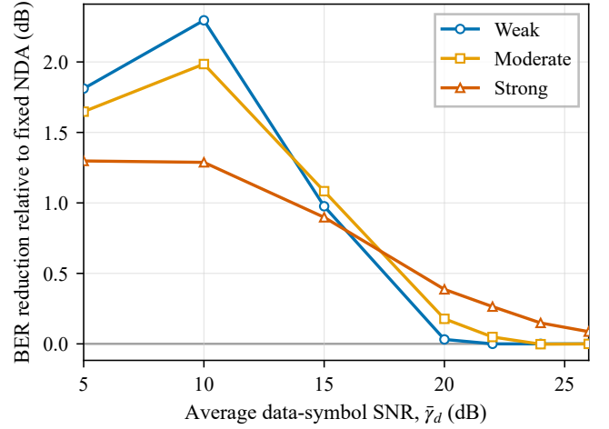
Fig. 5. Same-SNR BER reduction of the switched path relative to fixed NDA. G_{\text{BER}} = 10 \log_{10}(P_{b,\text{NDA}}/P_{b,\text{SW}}) , for weak, moderate, and strong downlink turbulence. Positive values indicate a lower switched-path BER at the same average data-symbol SNR and directly report the logarithmic BER ratio.
