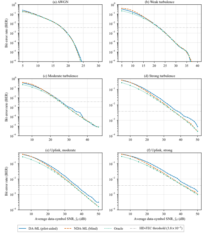
Fig. 3. BER versus average data-symbol SNR for DA-ML, NDA-ML, and the oracle reference under AWGN and five Gamma–Gamma turbulence conditions. Markers denote simulated samples and connecting curves are visual guides. Samples within 5–20 dB (AWGN) and 5–26 dB (turbulence) use 30 seeds with 400 blocks of 256 samples per seed; the high-SNR extension samples use five seeds. The horizontal dash-dotted line marks the 7% HD-FEC reference, P_b = 3.8 \times 10^{-3} .
