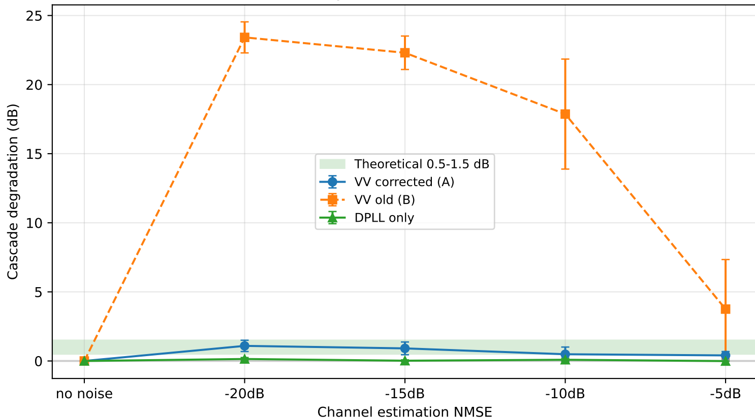
Weak Turbulence Cascade Degradation: Corrected vs Old VV (10 seeds x 100K symbols, SNR=20dB, fixed DPLL BW)
