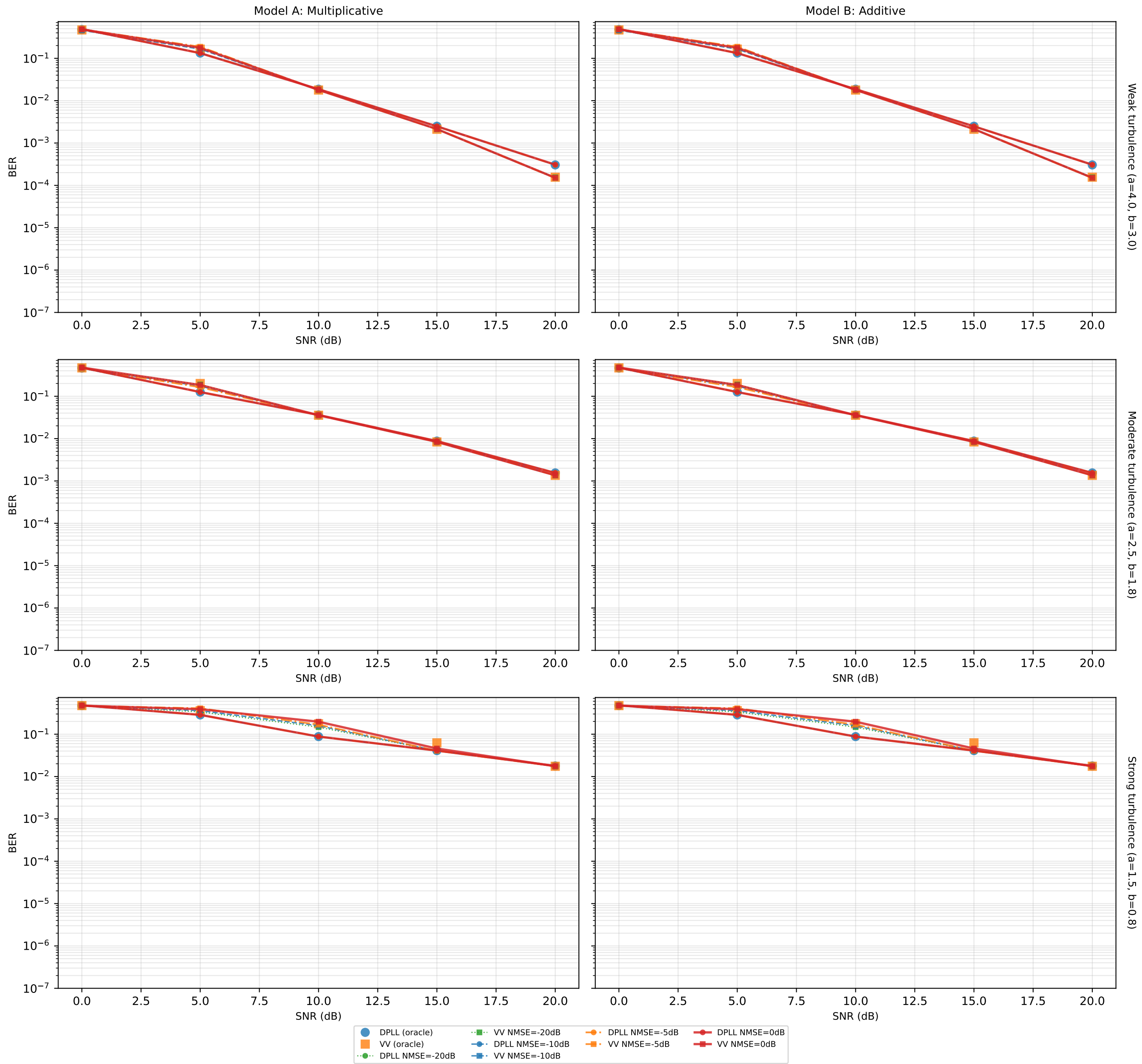
BER vs SNR under Channel Estimation Error — Turbulence Sweep
