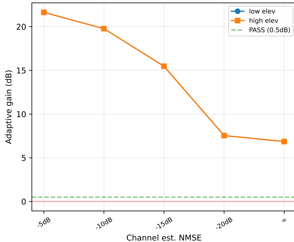
Weak turbulence
