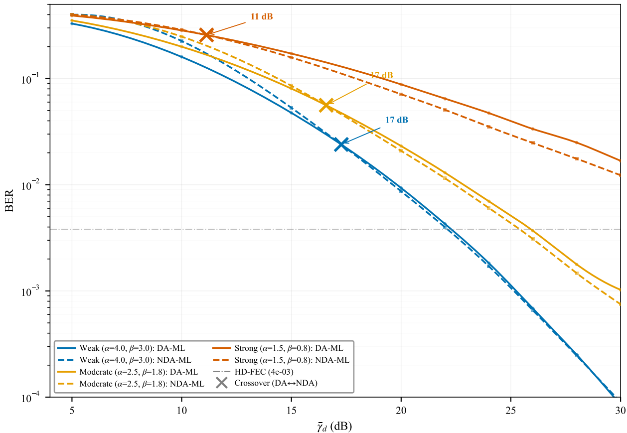
Crossover Shifts toward Lower SNR as Turbulence Strengthens
