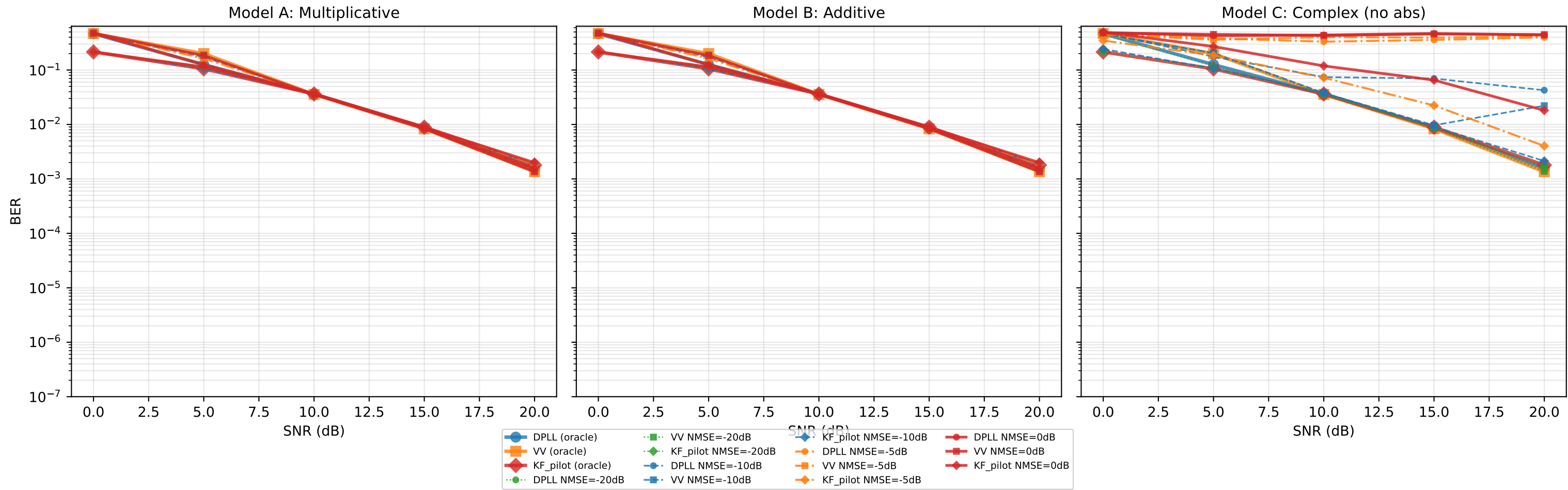
BER vs SNR under Channel Estimation Error (moderate turbulence)
