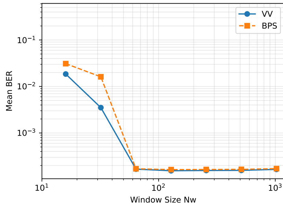
Weak Turbulence
