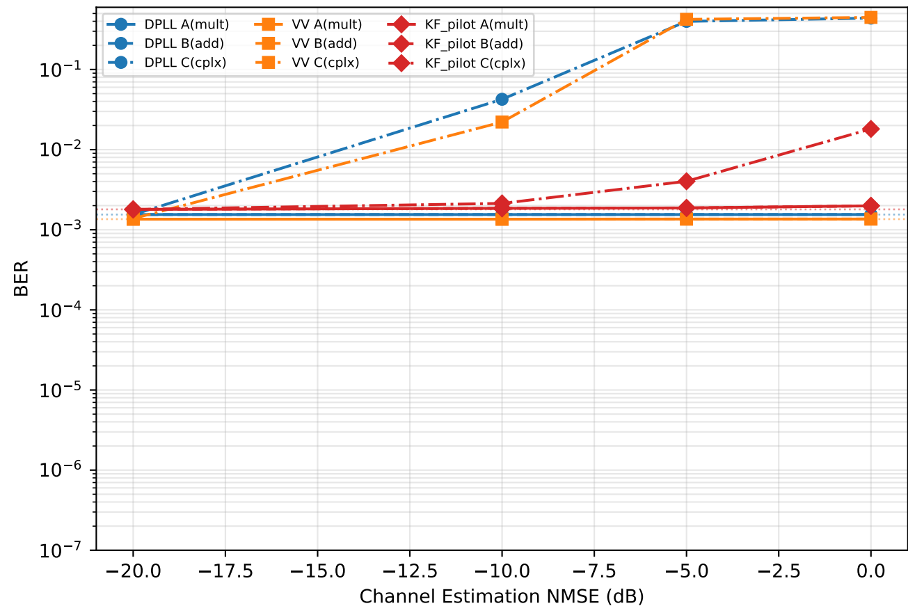
BER vs NMSE at SNR=20 dB (moderate turbulence)
